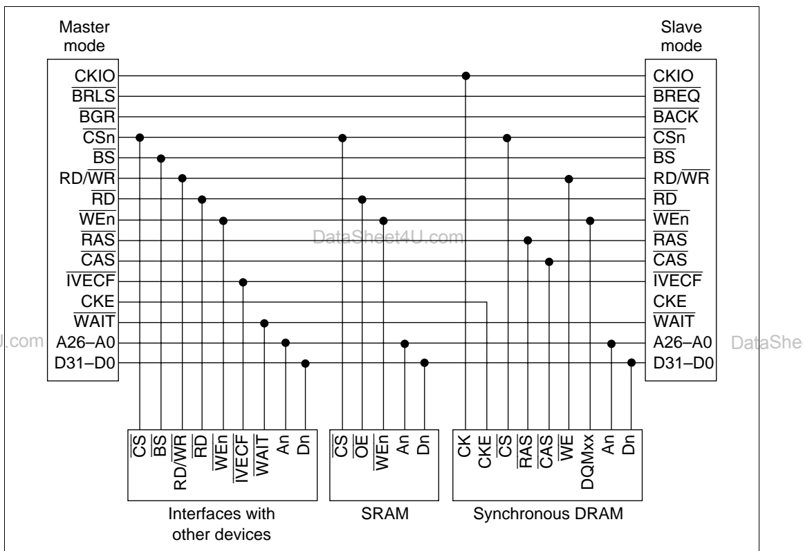
Figure 7.51 Connection between Master and Slave Devices
