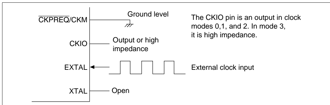
Figure 3.4 Inputting External Clock
