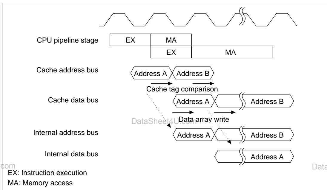
Figure 8.5 Write Access
