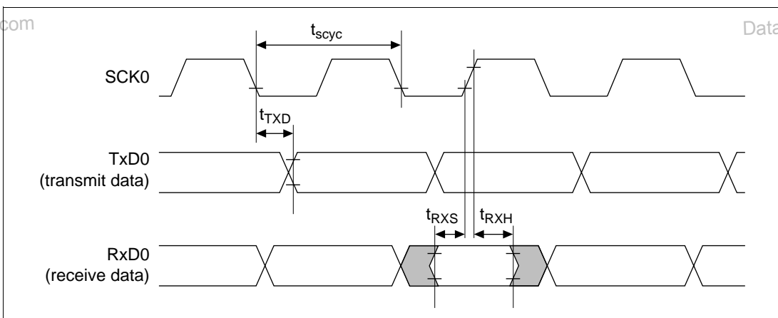
Figure 15.77 SCI Input/Output Timing (Clocked Synchronous Mode)
