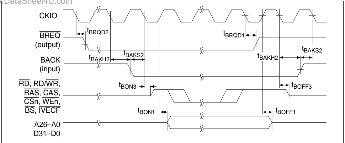
Figure 16.13 Bus Release Timing (Slave Mode, PLL1 Off)
