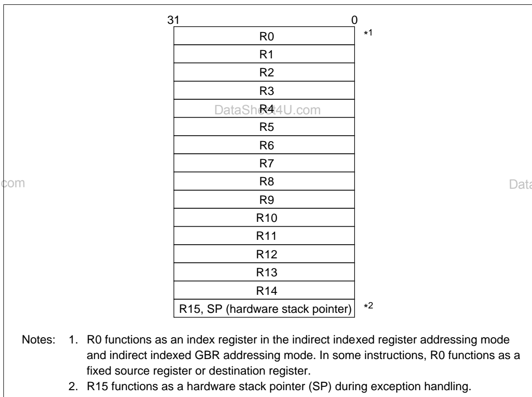
Figure 2.1 General Registers
