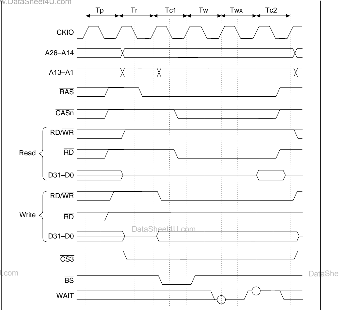
Figure 7.33 External Wait State Timing
