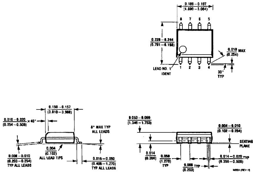
SO Package (M) Order Number LF351M NS Package Number M08A
