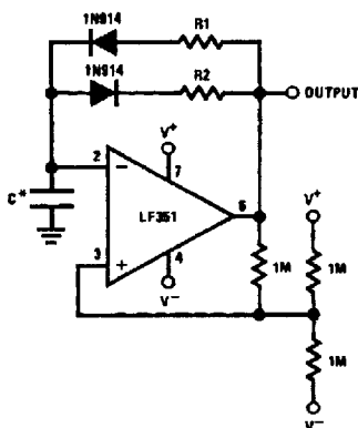
Ultra-Low (or High) Duty Cycle Pulse Generator
