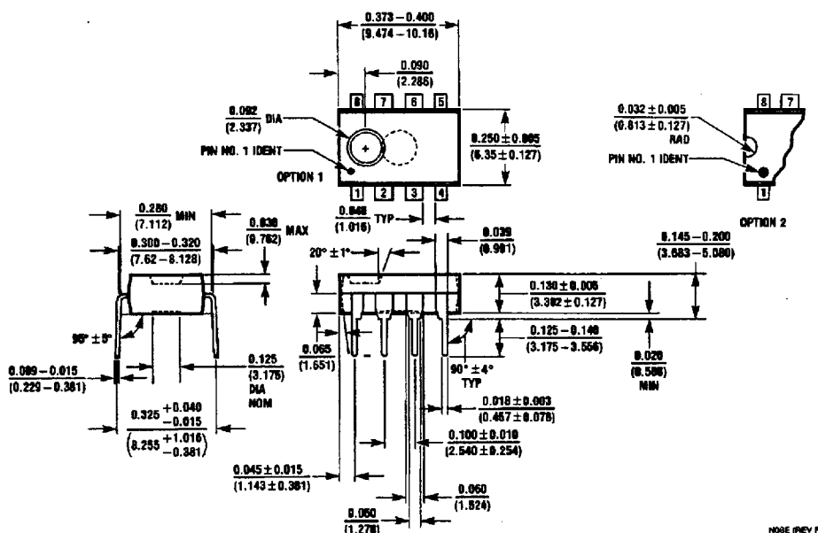
Molded Dual-In-Line Package (N) Order Number LF351N NS Package Number N08E
