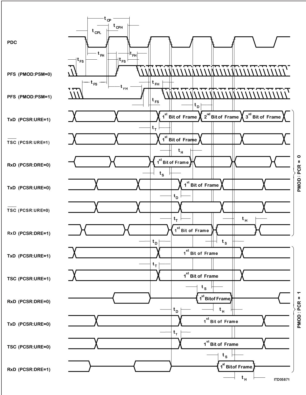
Figure 24 PCM-Interface Timing
