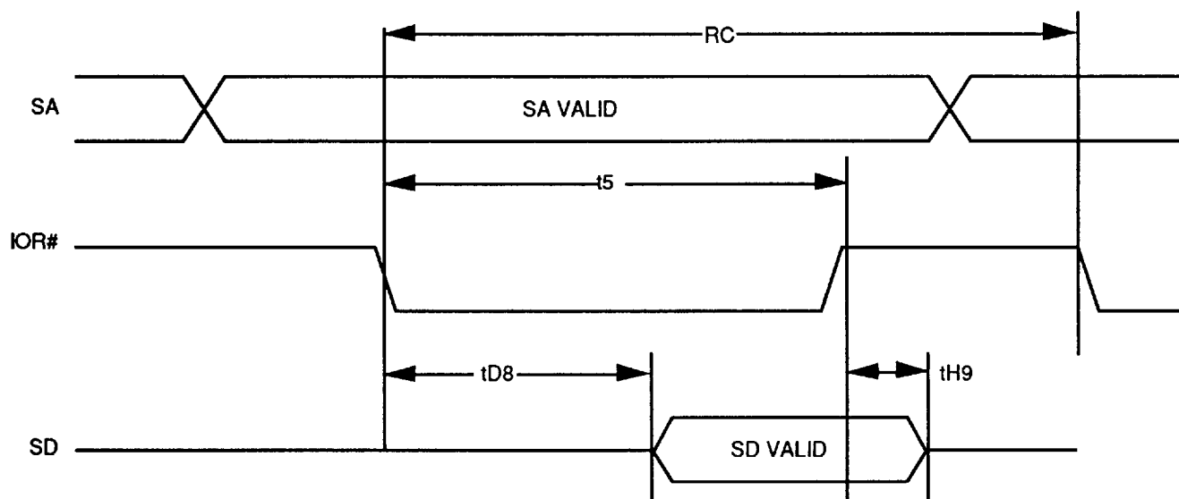
FIGURE 3. READ CYCLE TIMING
