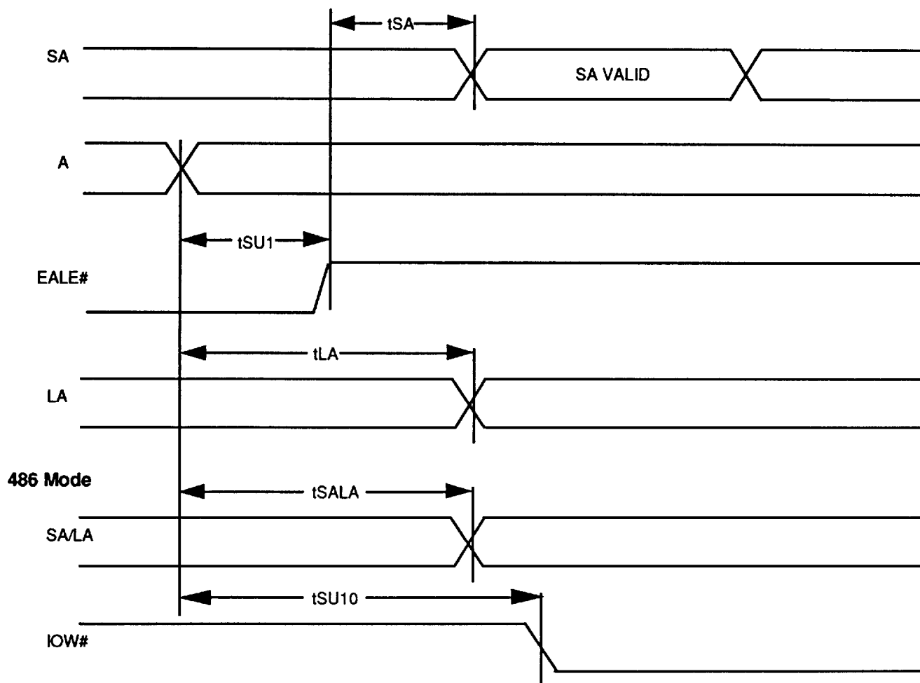
FIGURE 2. WRITE CYCLE TIMING (2)
