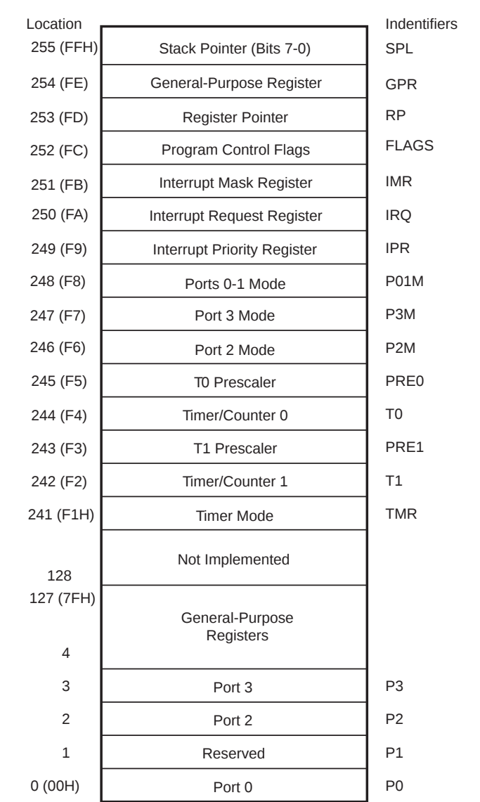
Figure 12. Register File
