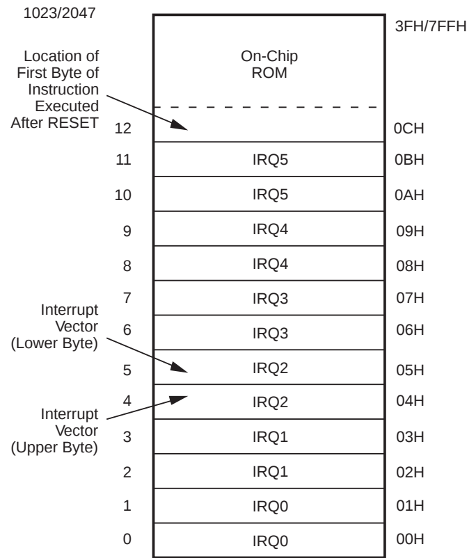
Figure 11. Program Memory Map
