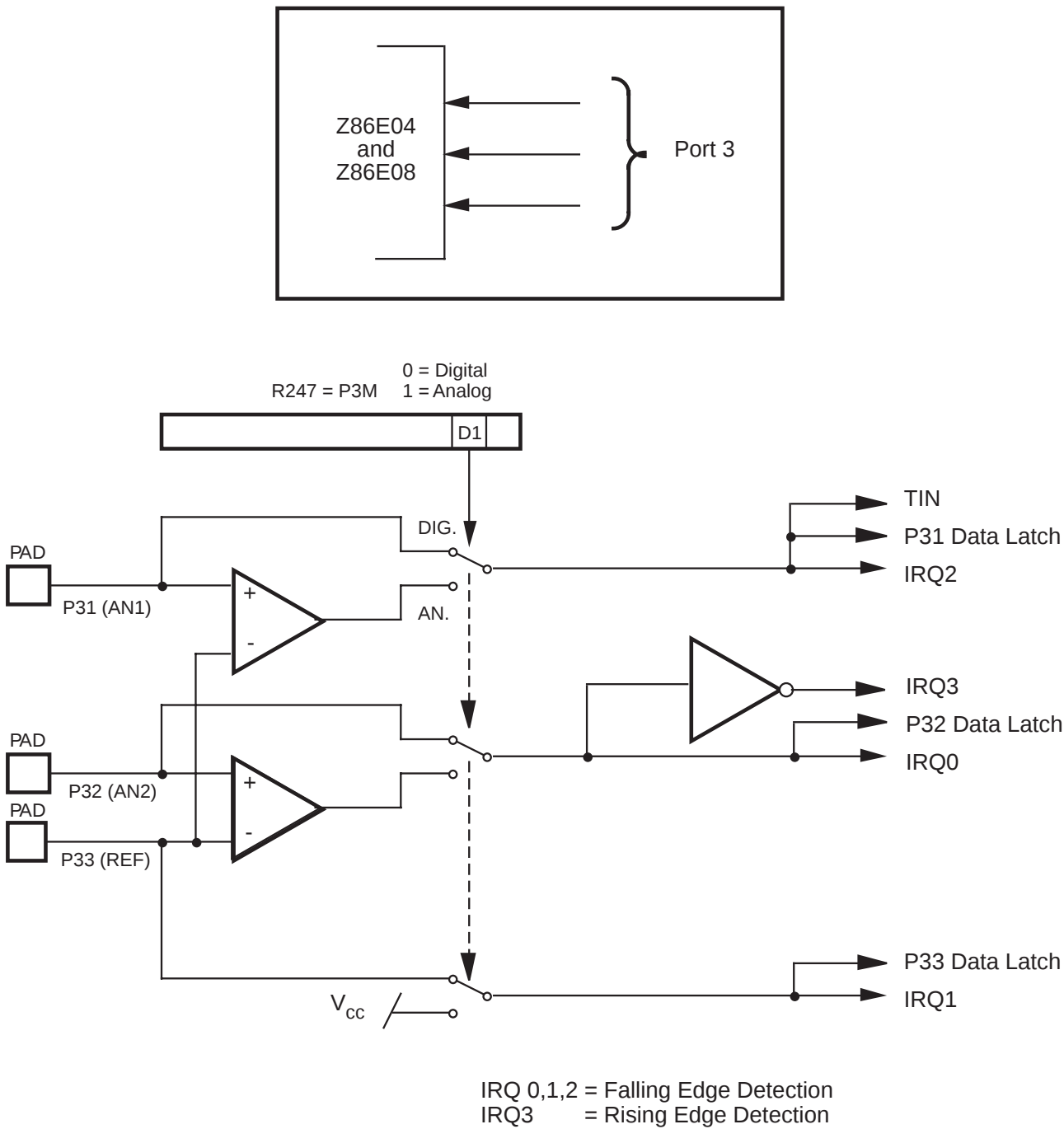
Figure 9. Port 3 Configuration
