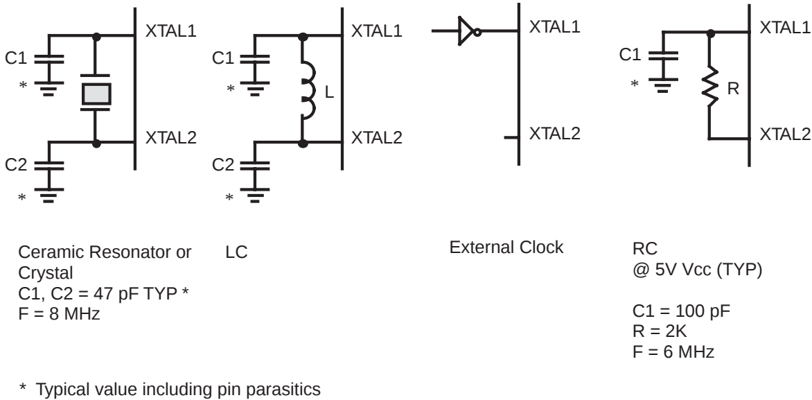
Figure 16. Oscillator Configuration
