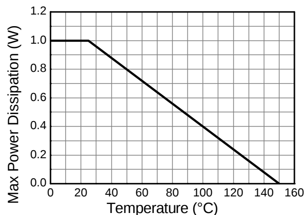
Derating Curve
