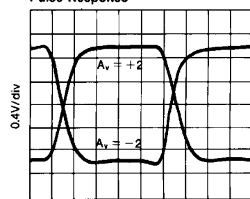
Pulse Response
