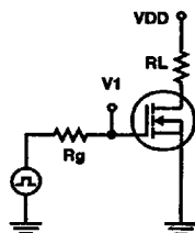
FIGURE 1. SWITCHING TIME TESTING
