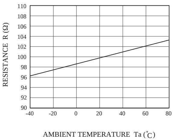
R_{Line} - TEMPERATURE
