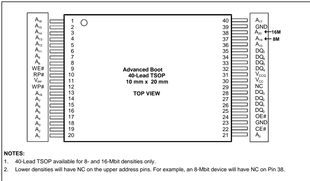
Figure 1. 40-Lead TSOP Package for x8 Configurations
