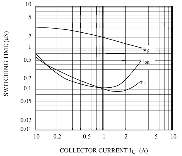
SWITCHING CHARACTERISTICS
