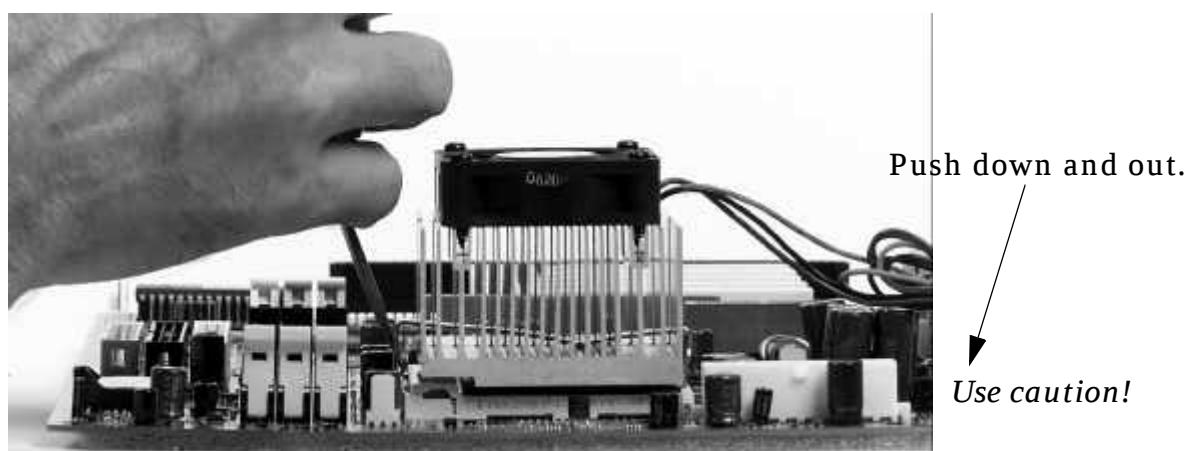
Figure 16. Pushing the Clip Past the Socket Lug
