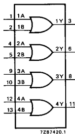
Fig. 2 Logic symbol.
