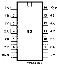
Fig. 1 Pin configuration.
