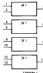
Fig. 3 IEC logic symbol.
