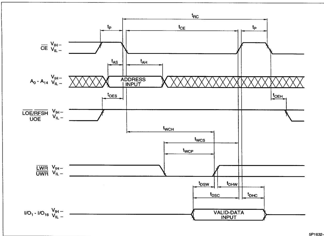
Figure 4. Write Cycle
