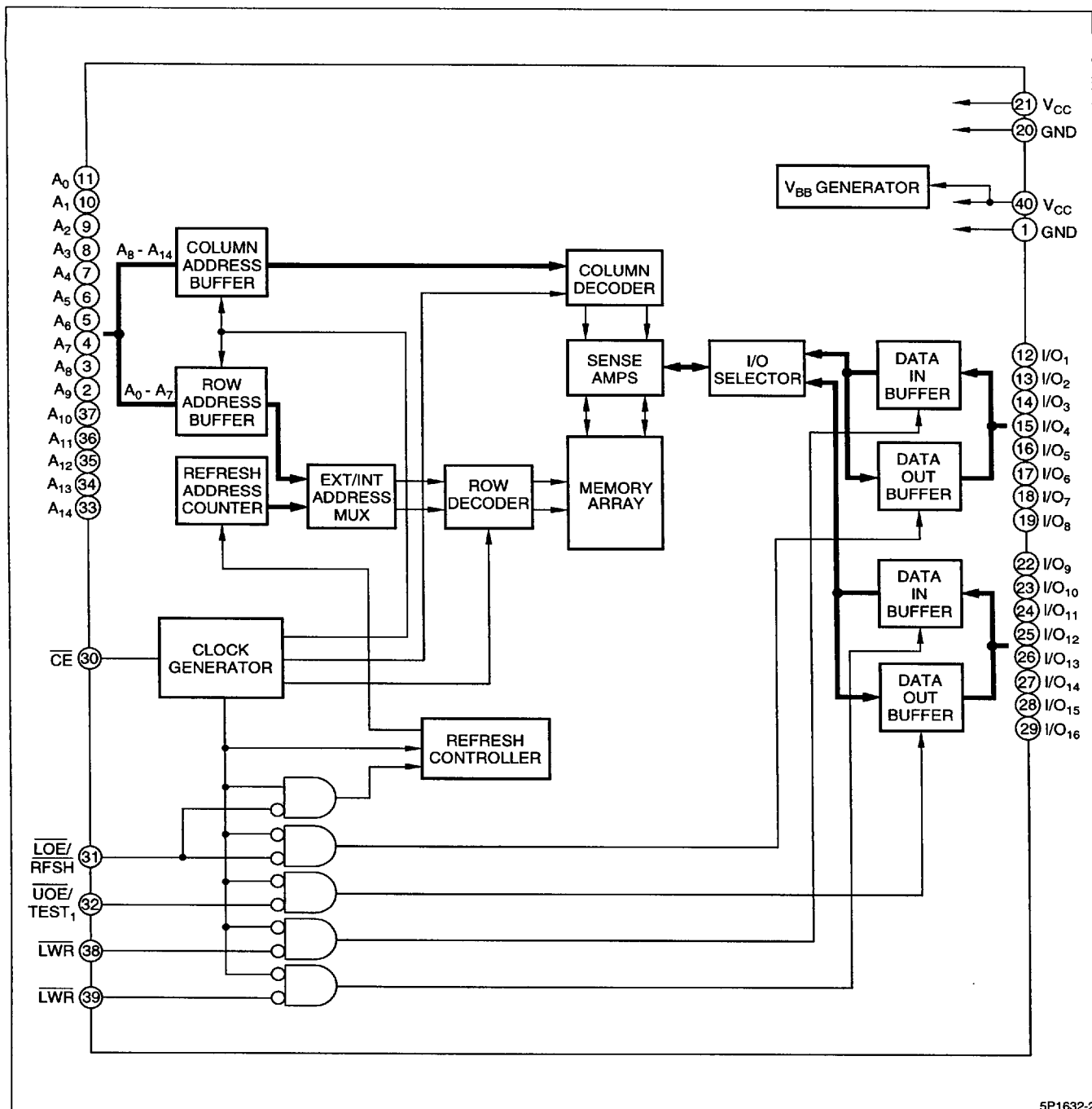
Figure 2. LH5P1632 Block Diagram
