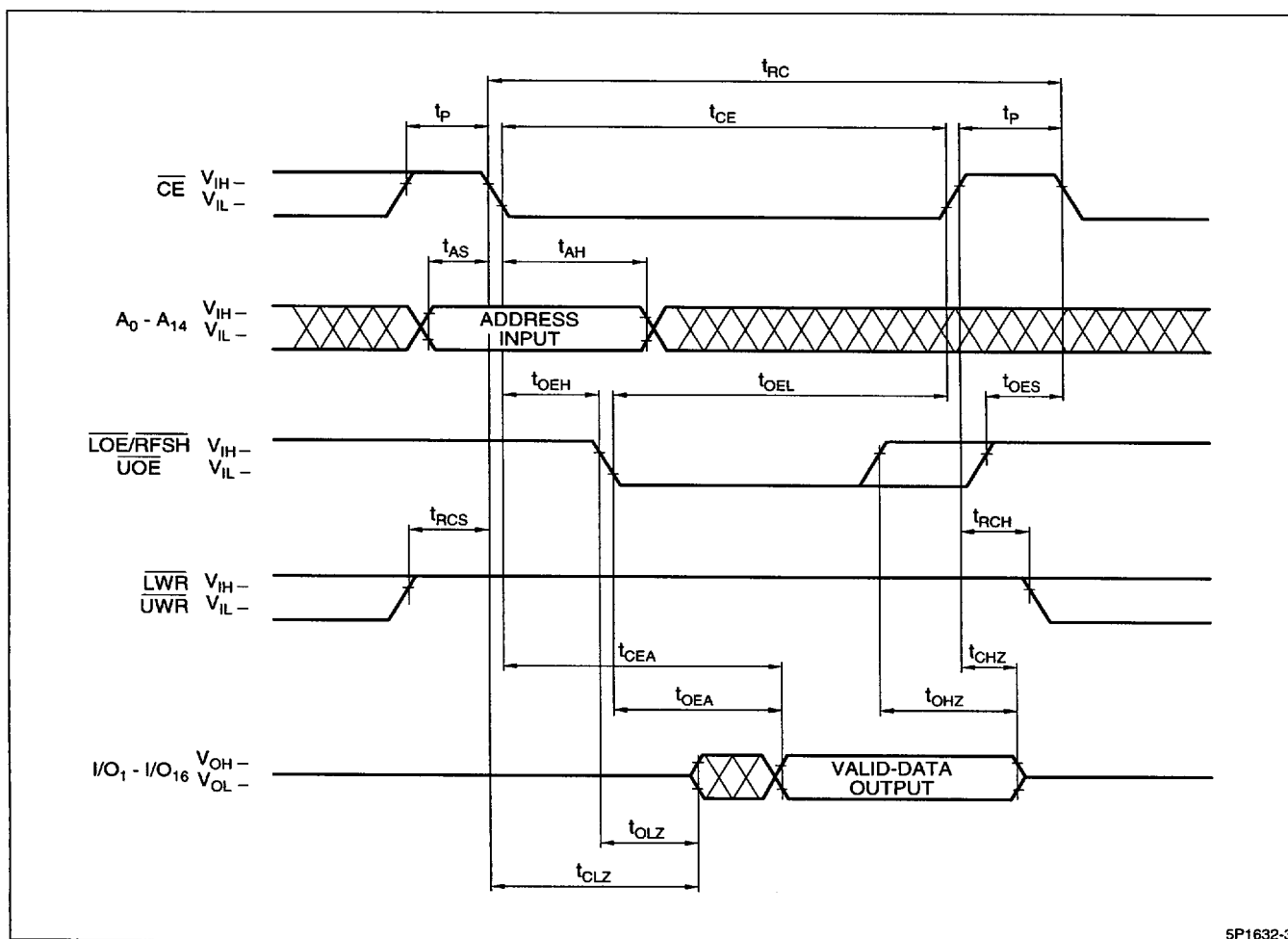
Figure 3. Read Cycle
