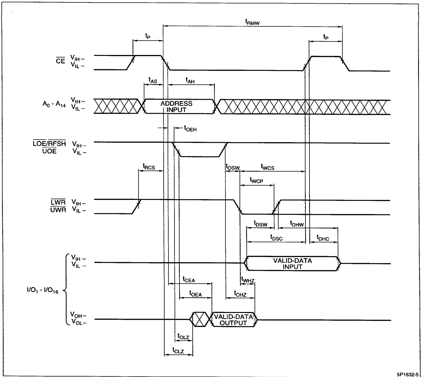
Figure 5. Read-Write Cycle
