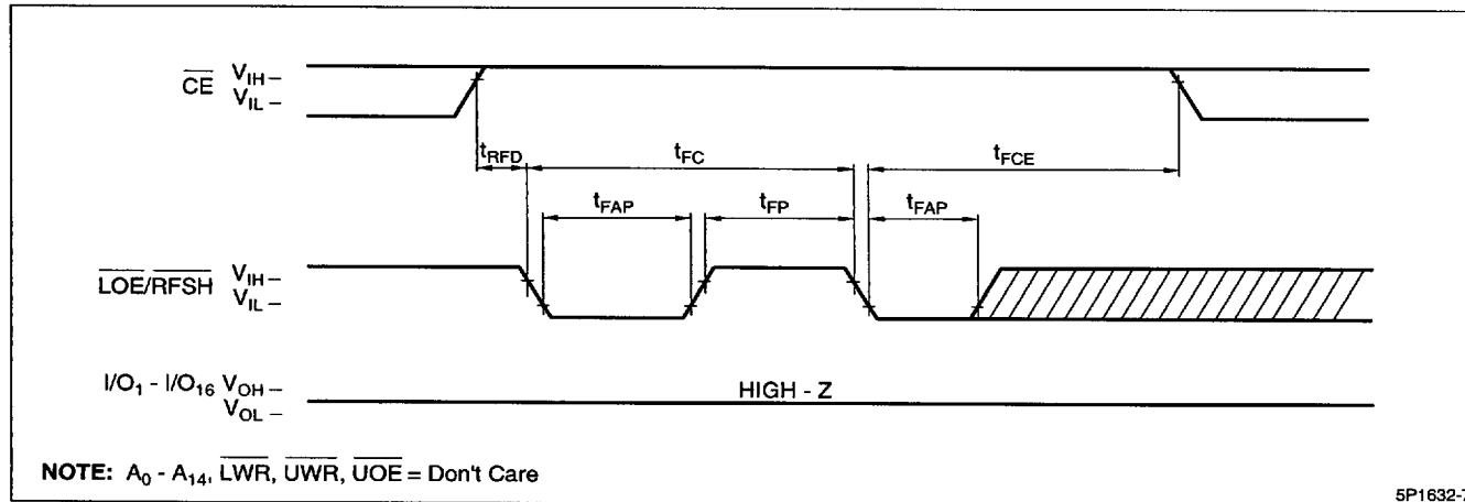
Figure 7. Auto Refresh Cycle
