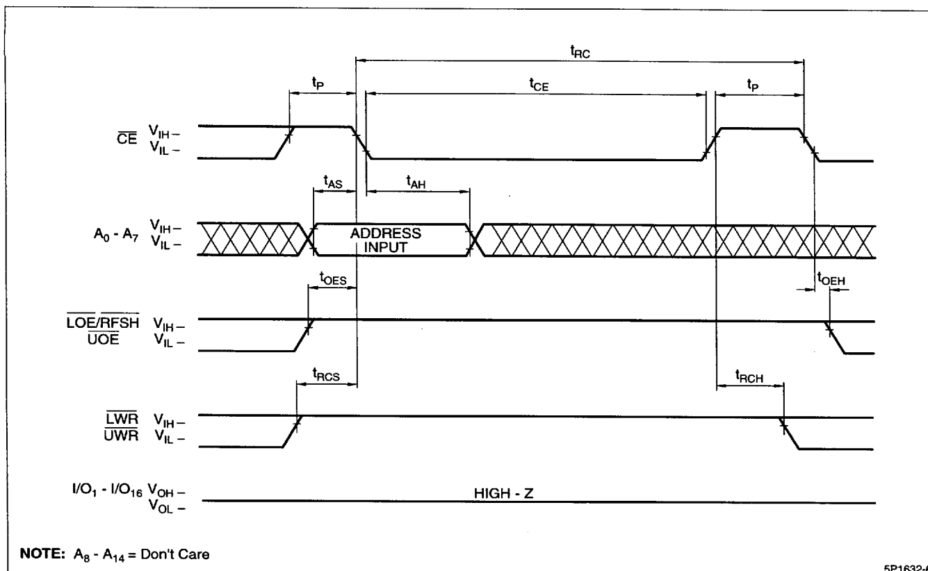
Figure 6. CE Only Refresh Cycle
