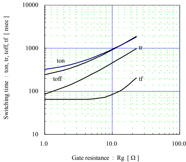
Switching time vs. Gate resistance (typ.) V_{cc}=300V , I_c=600A , V_{GE}=\pm 15V , T_j=25^\circ C
