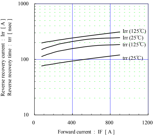
Reverse recovery characteristics (typ.) Vcc=300V, VGE=±15V, Rg=4.7Ω
