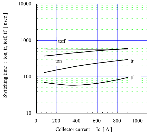
Switching time vs. Collector current (typ.) V_{cc}=300V , V_{GE}=\pm 15V , R_g=4.7\Omega , T_j=25^\circ C
