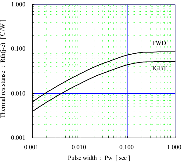
a Transient thermal resistance (max.)
