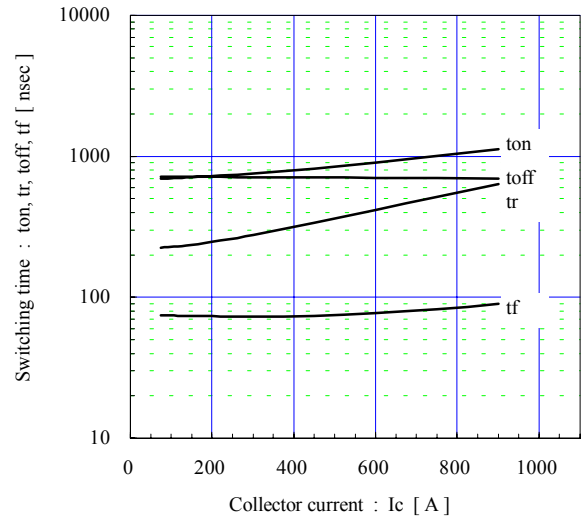
Switching time vs. Collector current (typ.) V_{cc}=300V , V_{GE}=\pm 15V , R_g=4.7\Omega , T_j=125^\circ C
