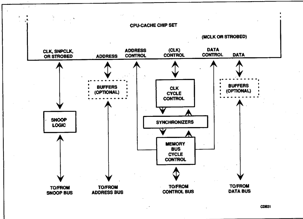
Figure 5-1. MBC Block Diagram
