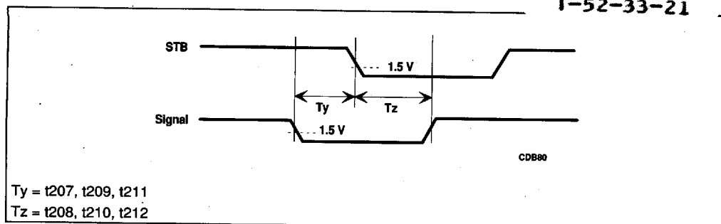
Figure 7-11. Setup and Hold Timings to Strobes
