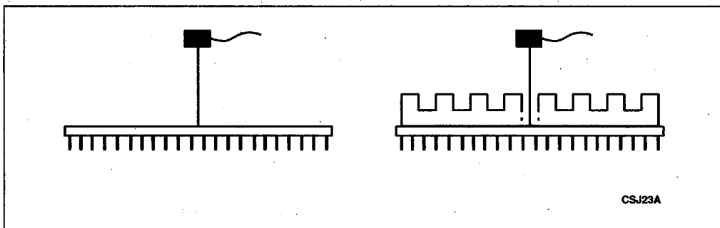
Figure 10-1. Technique For Measuring Tcase
