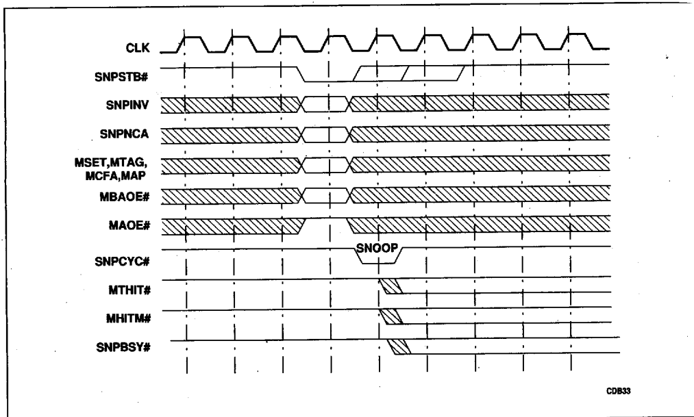
Figure 5-4. Synchronous Snoop Mode
