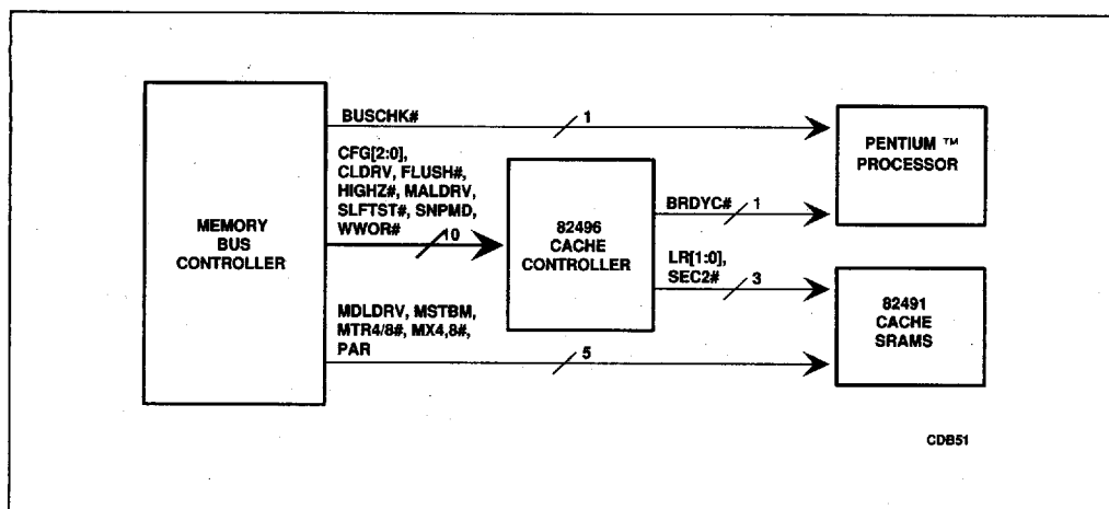
Figure 4-3. CPU-Cache Chip Set Configuration Inputs
