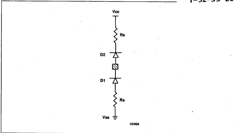
Figure 8-3. Input Diode Model
