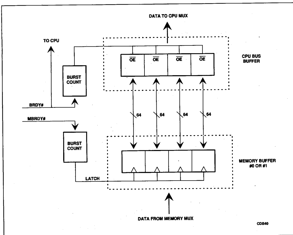
Figure 5-20. 82491 Cache SRAM Read Data Path
