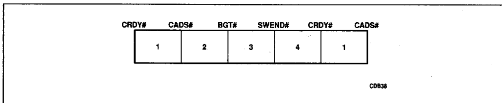
Figure 5-12. Snoop Response During Cycles
