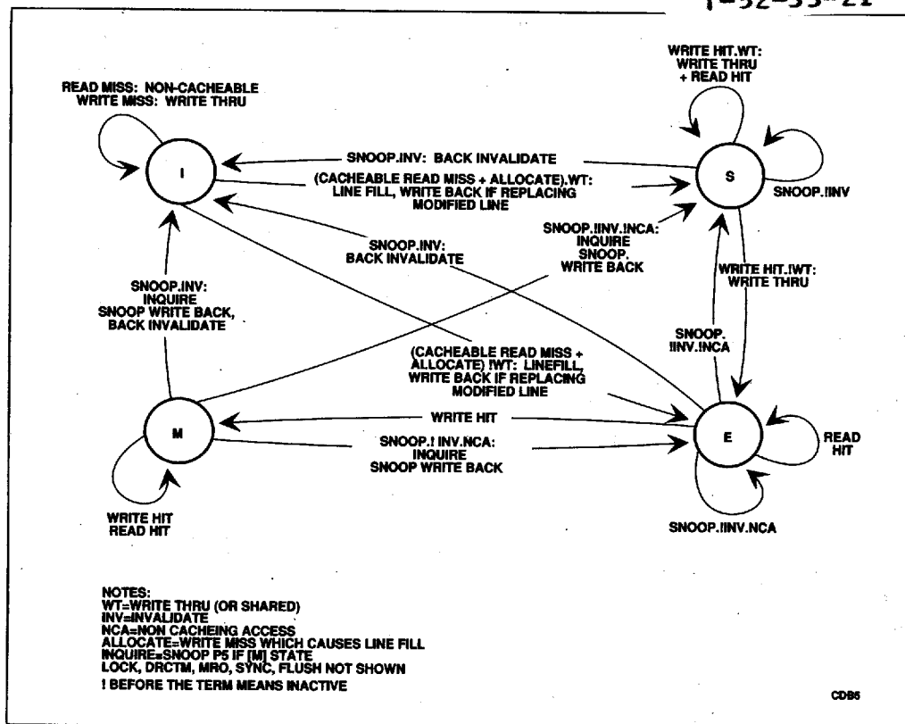
Figure 3-1. State Changes
