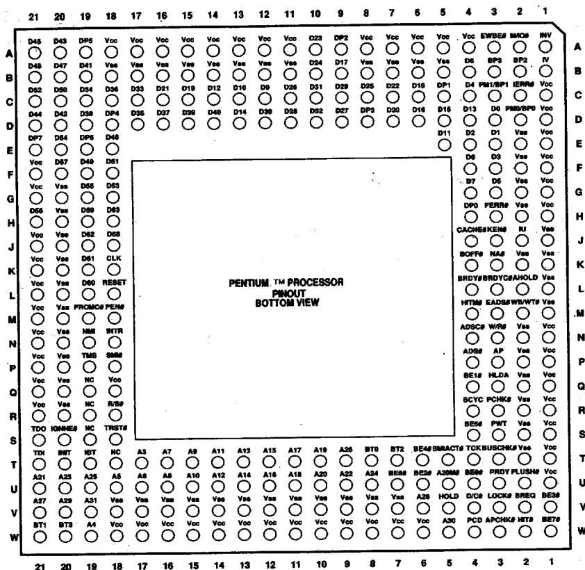
Figure 1-2. Pentium™ Processor Pinout (Bottom View)
