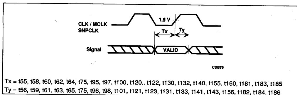
Figure 7-7. Setup and Hold Timings
