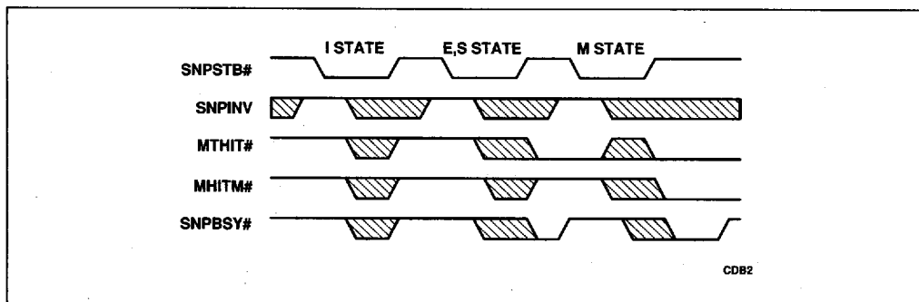
Figure 5-11. Snoops with Invalidation
