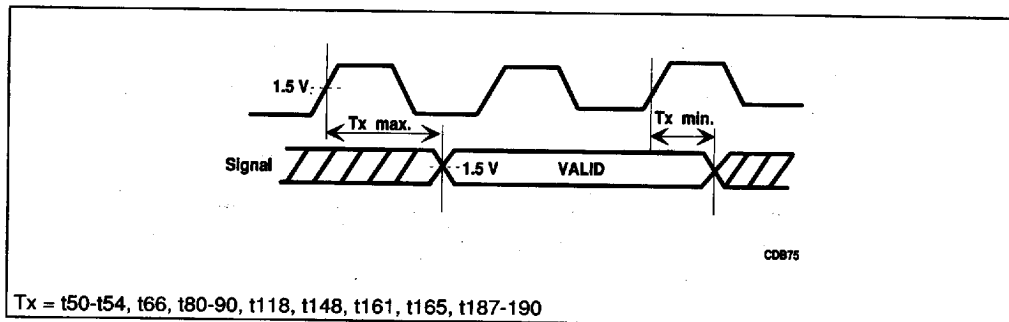
Figure 7-6. Valid Delay Timings
