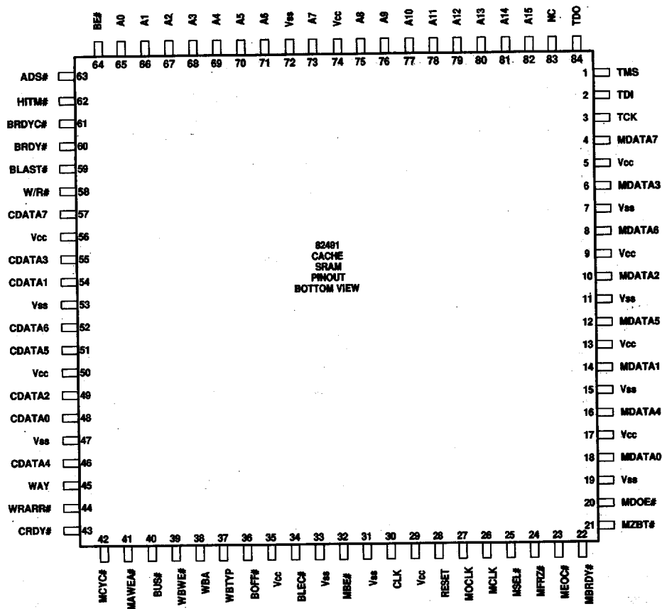
Figure 1-6. 82491 Cache SRAM Pinout (Bottom View)
