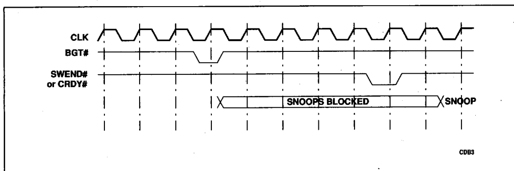
Figure 5-13. Snoop Response Blocking Using BGT#
