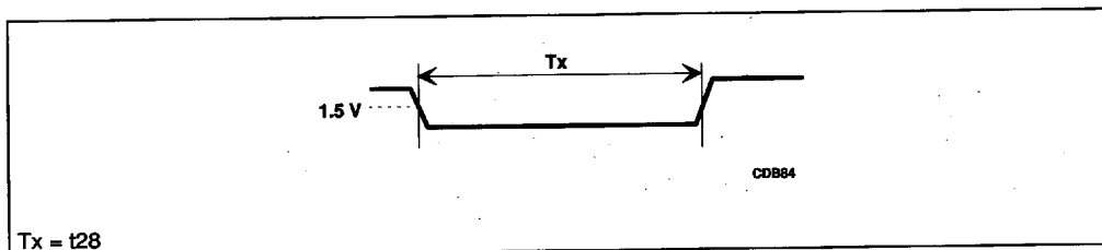
Figure 7-15. Test Reset Timings
