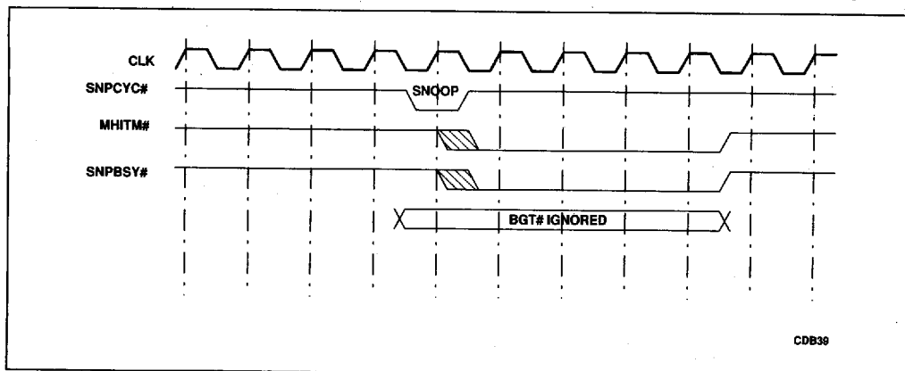
Figure 5-14. Snoop Executing before BGT# Is Asserted
