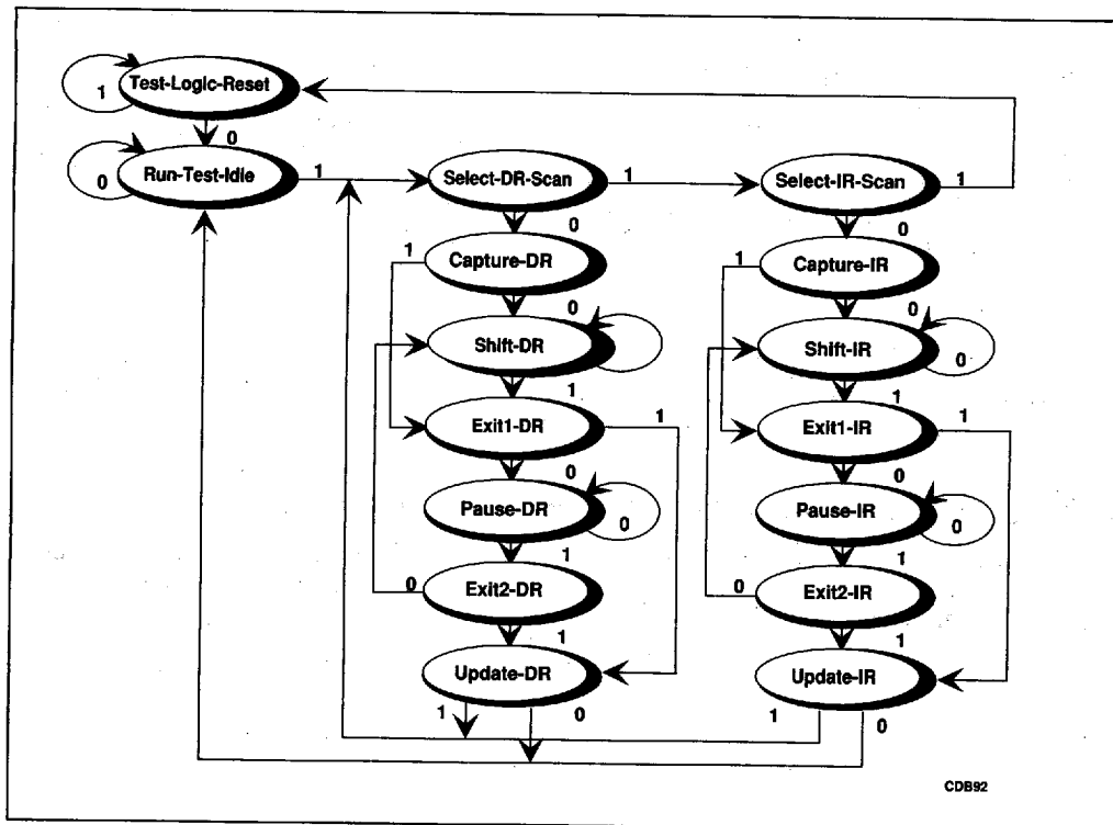
Figure 11-3. TAP Controller State Diagram
