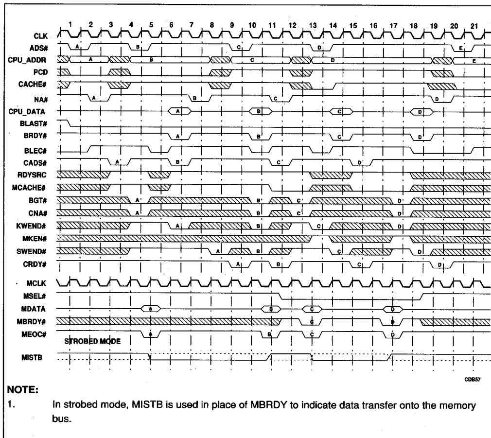
Figure 6-4. Non Cacheable Read Miss
