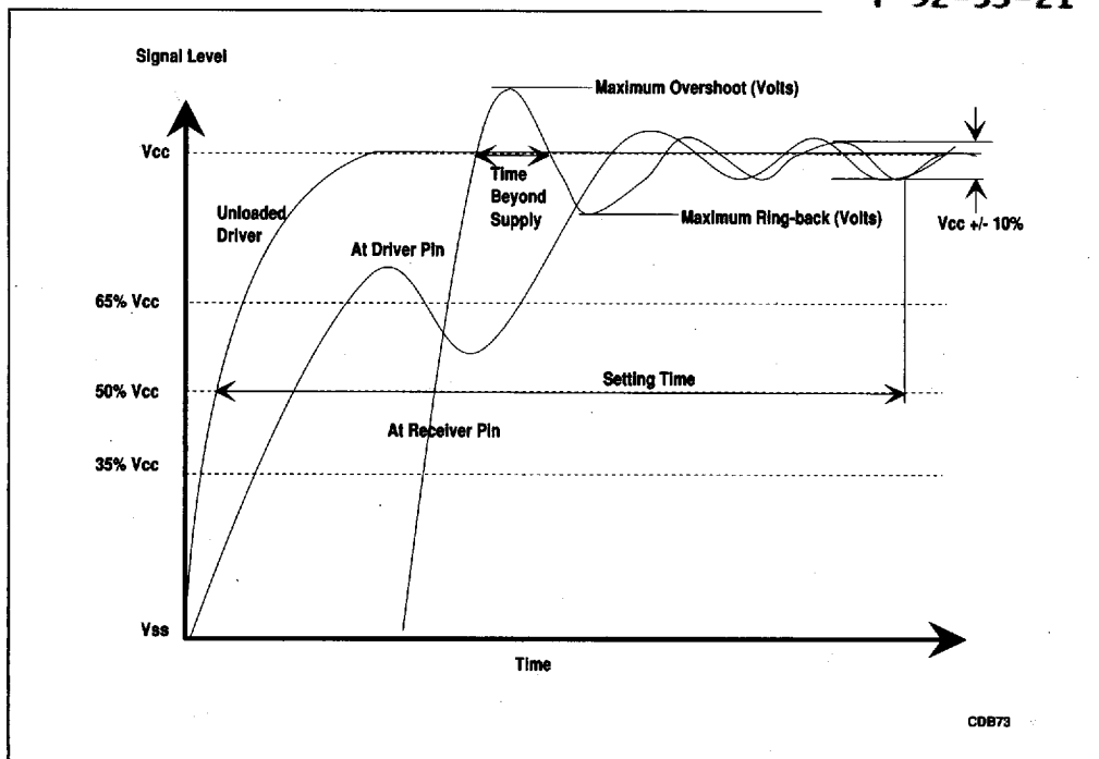
Figure 7-4. Driver and Receiver Signal Waveforms Showing Signal Quality Parameters
