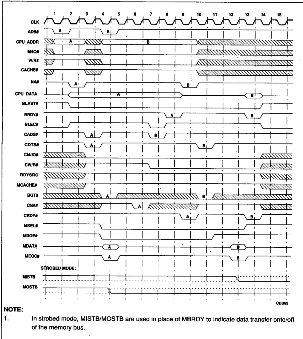
Figure 6-10. I/O Cycles
