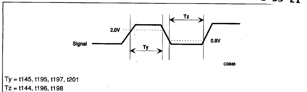
Figure 7-16. Active/Inactive Timings
