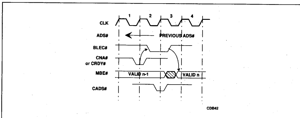
Figure 5-24. BLEC# Assertion Due to CNA# or CRDY# Assertion
