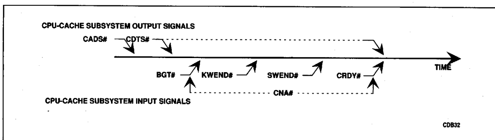
Figure 5-3. Cycle Progress Signals and Responses
