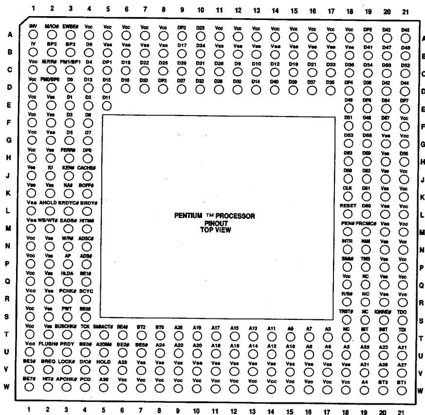
Figure 1-1. Pentium™ Processor Pinout (Top View)
