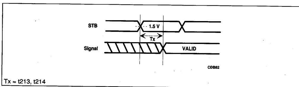
Figure 7-13. Valid Delay Timings from Strobes
