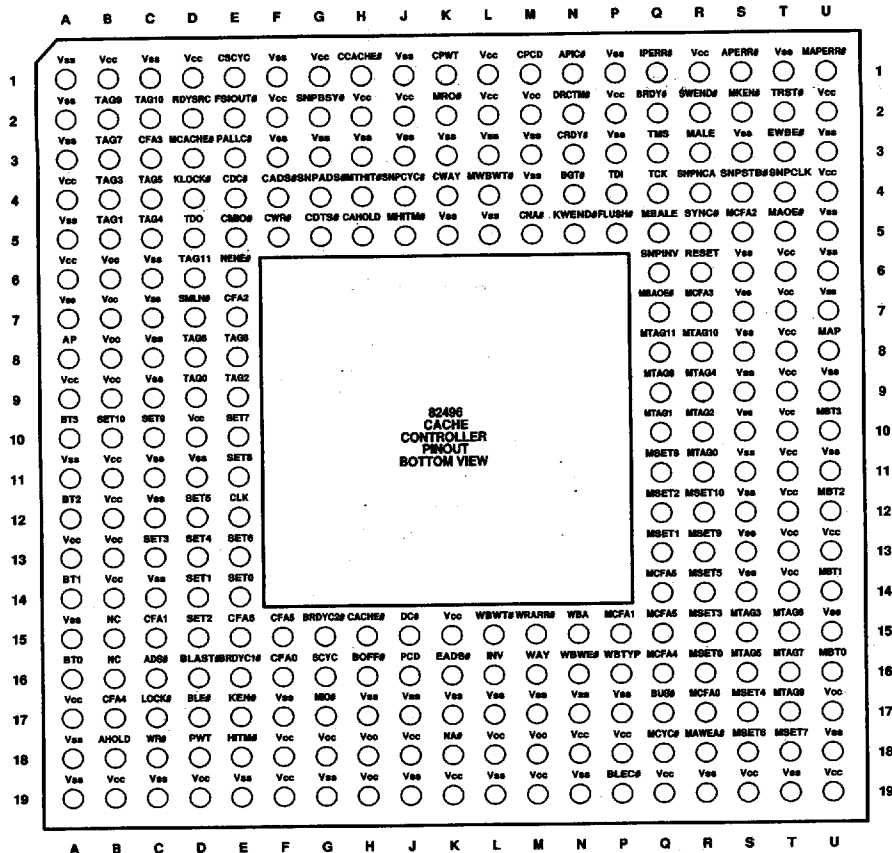
Figure 1-4. 82496 Cache Controller Pinout (Bottom View)
