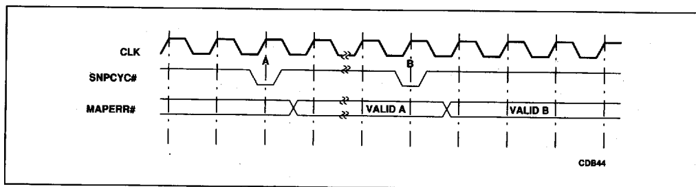
Figure 5-18. MAPERR# Timing for Asynchronous Snoop Modes
