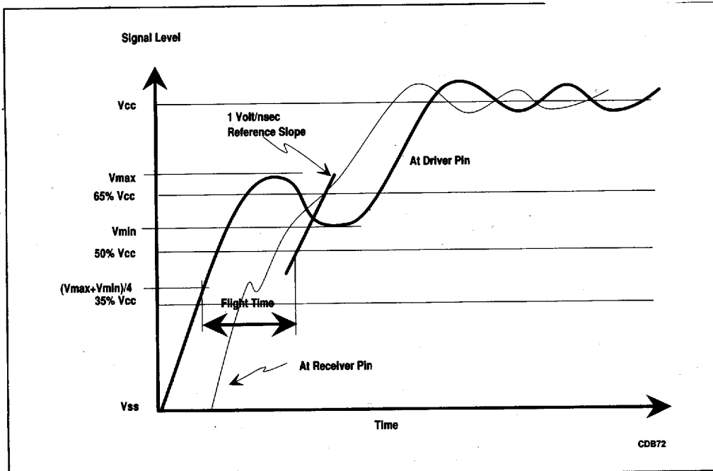
Figure 7-3. In-System Measurement of Flight Time
