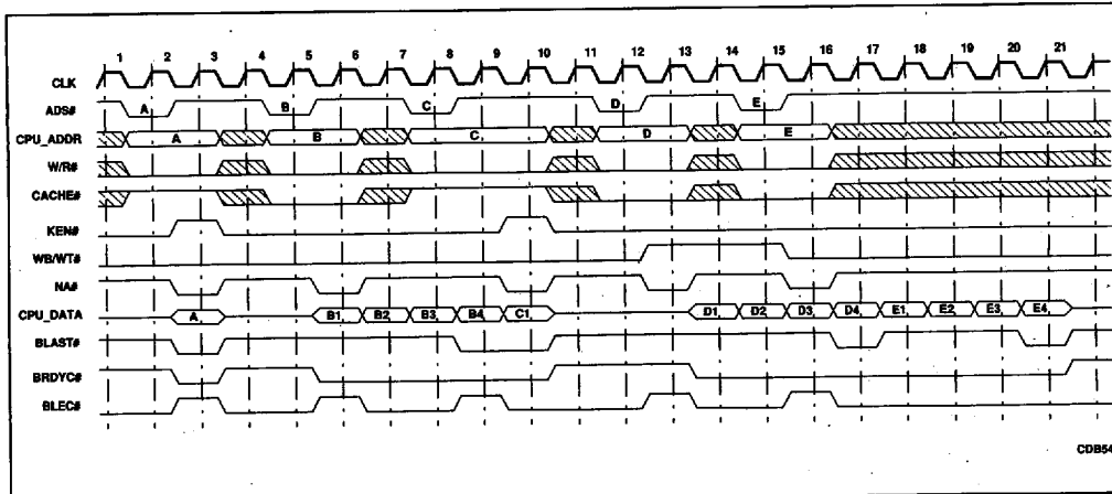
Figure 6-1. Pipelined Read Hits
