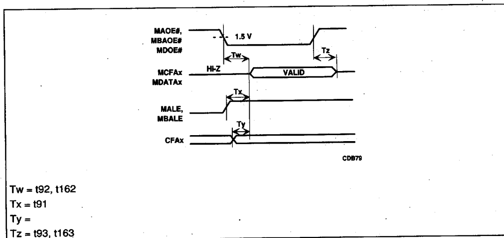
Figure 7-10. Memory Interface Timings
