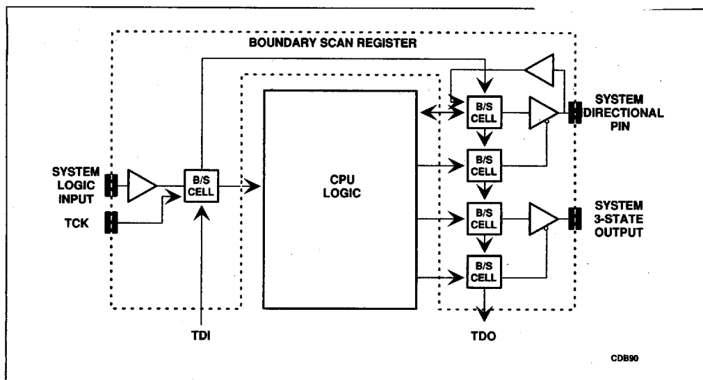
Figure 11-1. Boundary Scan Register Structure of a Component
