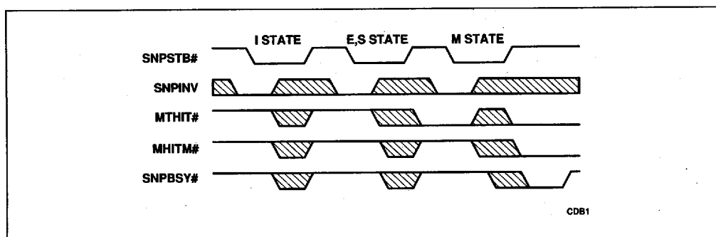
Figure 5-10. Snoops without Invalidation
