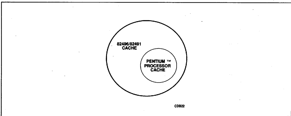
Figure 3-2. Pentium™ Processor CPU-Cache Chip Set Cache Inclusion
