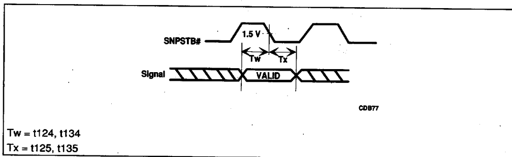
Figure 7-8. Setup and Hold Timings in Strobed Snooping Mode
