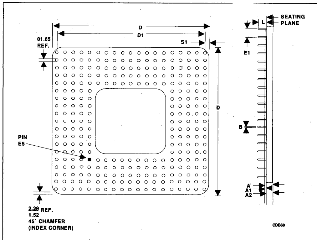
Figure 9-2. 82496 Cache Controller Mechanical Specifications
