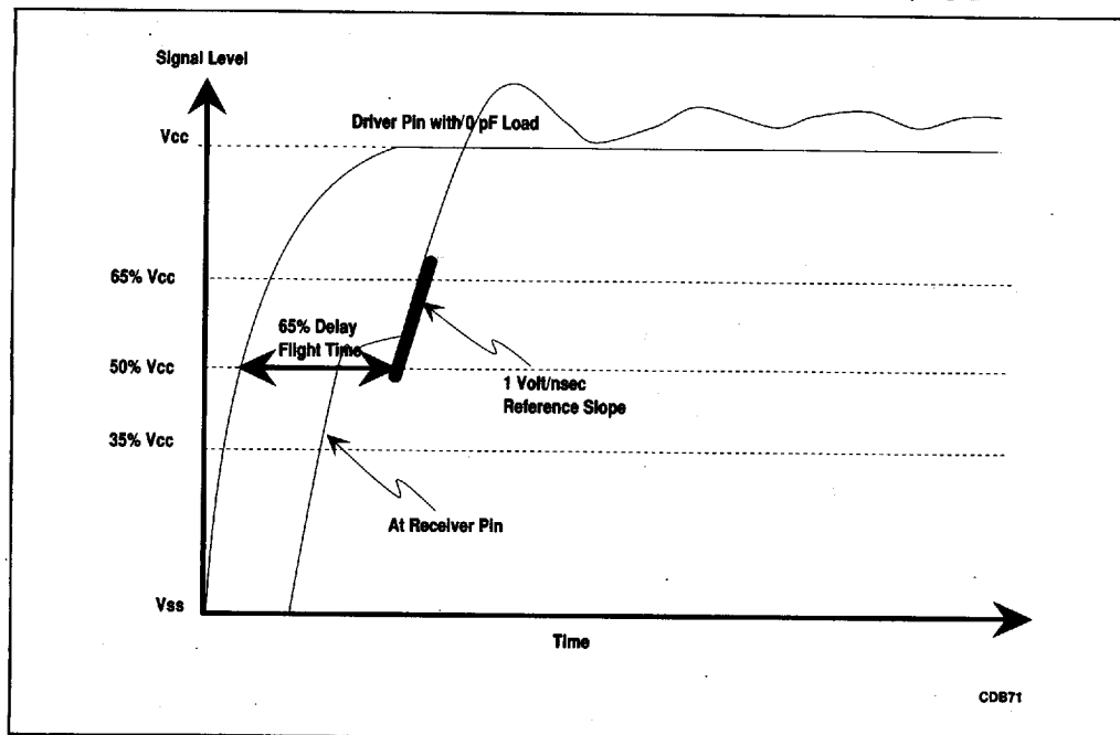
Figure 7-2. Derating the Flight Time
