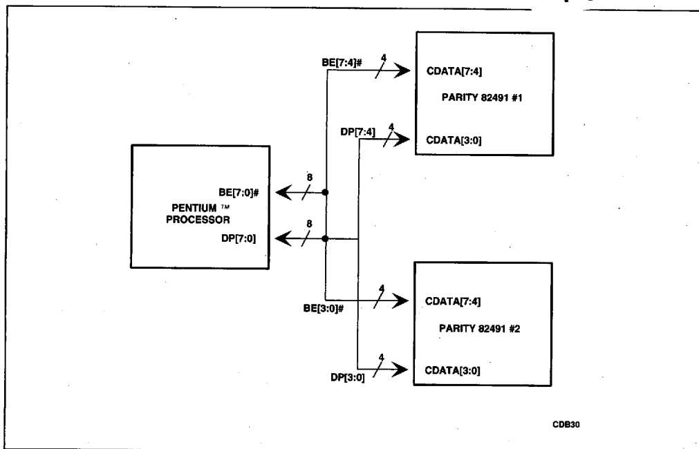
Figure 5-21. Pentium™ Processor/82491 Cache SRAM Data Parity Connections
