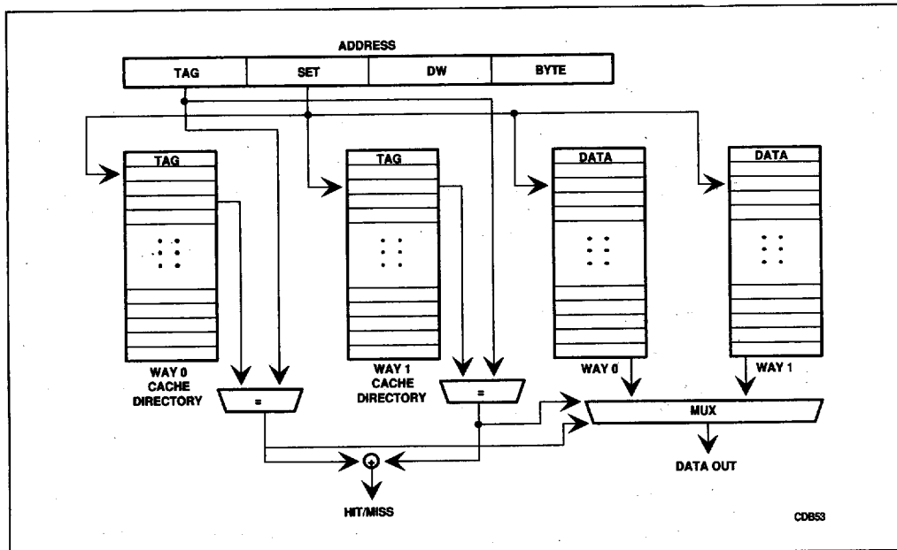
Figure 4-4. Two-Way Set Associative TagRAM Structure
