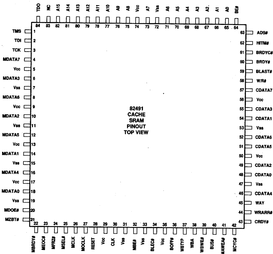
Figure 1-5. 82491 Cache SRAM Memory Pinout (Top View)
