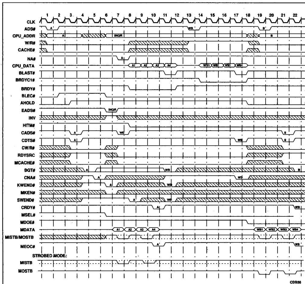
Figure 6-3. Read Miss with Replacement of Modified Line
