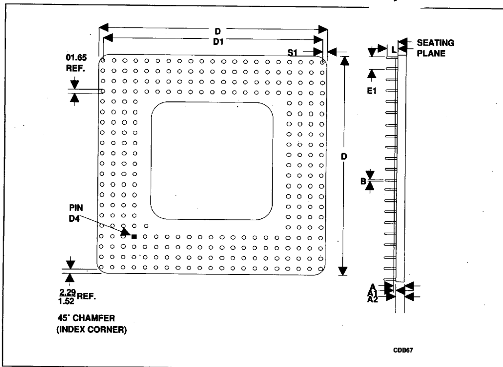
Figure 9-1. Pentium™ Processor Mechanical Specifications
