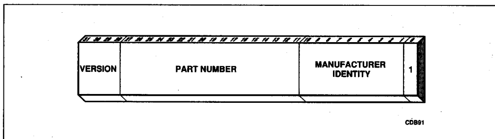
Figure 11-2. Device ID Register
