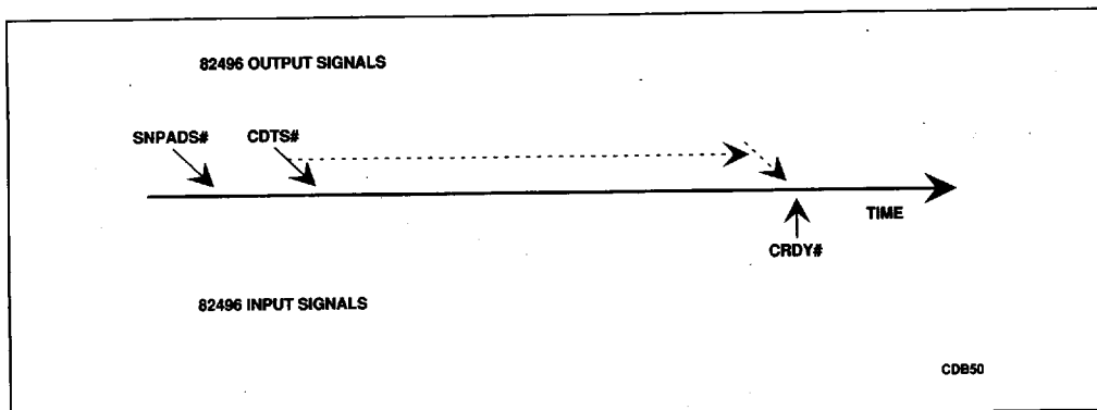
Figure 5-16. Cycle Progress for Snoop Write Back Cycles
