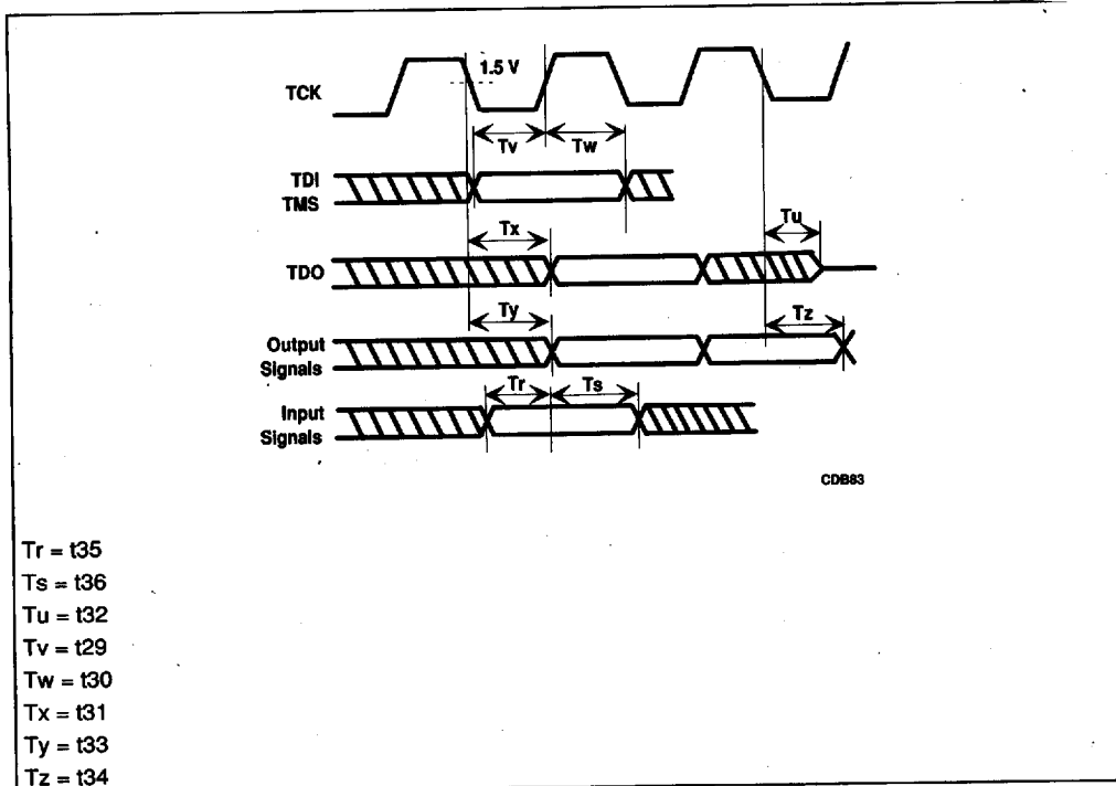
Figure 7-14. Test Timings
