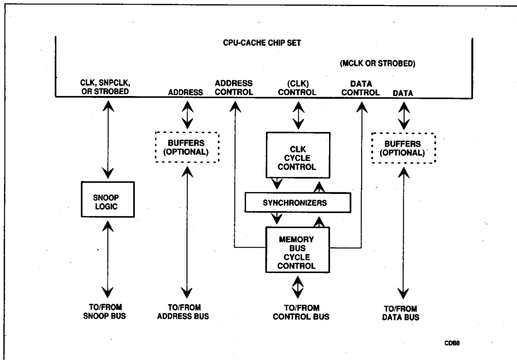
Figure 2-3. MBC Block Diagram
