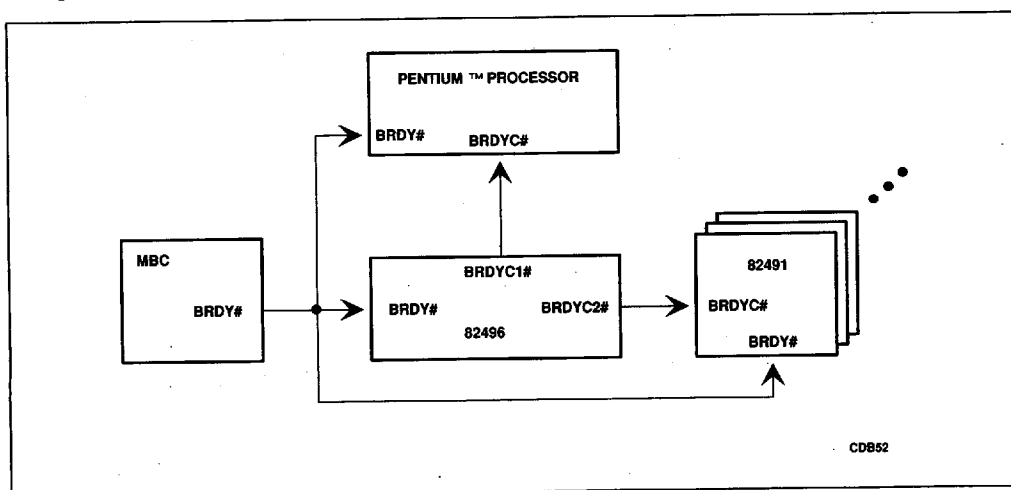
Figure 5-19. BRDY# / BRDYC# / BRDYC1# / BRDYC2# Interconnection
