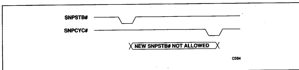
Figure 5-15. New SNPSTB# Not Allowed
