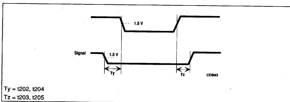
Figure 7-12. Setup and Hold Timings M_xST
