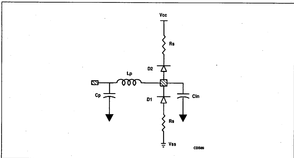
Figure 8-4. Complete Input Model Including Diode
