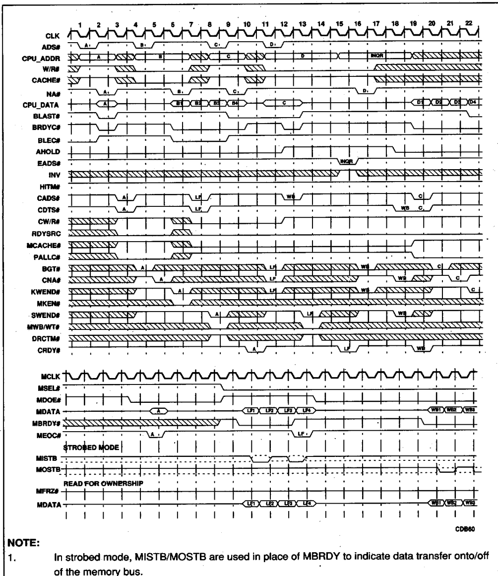
Figure 6-7. Write Miss with Allocation to Modified Line
