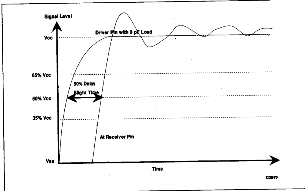
Figure 7-1. Determination of Flight Time
