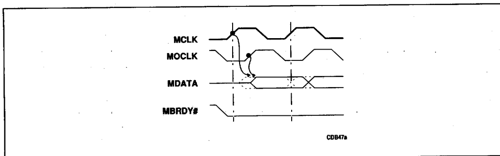
Figure 5-29. Increasing Hold Time of Output Burst Data
