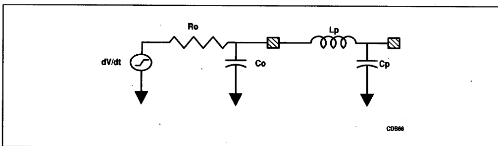
Figure 8-2. First Order Output Buffer
