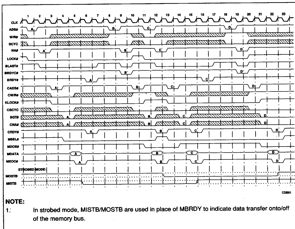
Figure 6-8. Locked Read Modify Write Cycles
