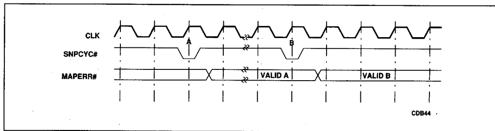
Figure 5-27. MBE# [PAR#] Timing After RESET
