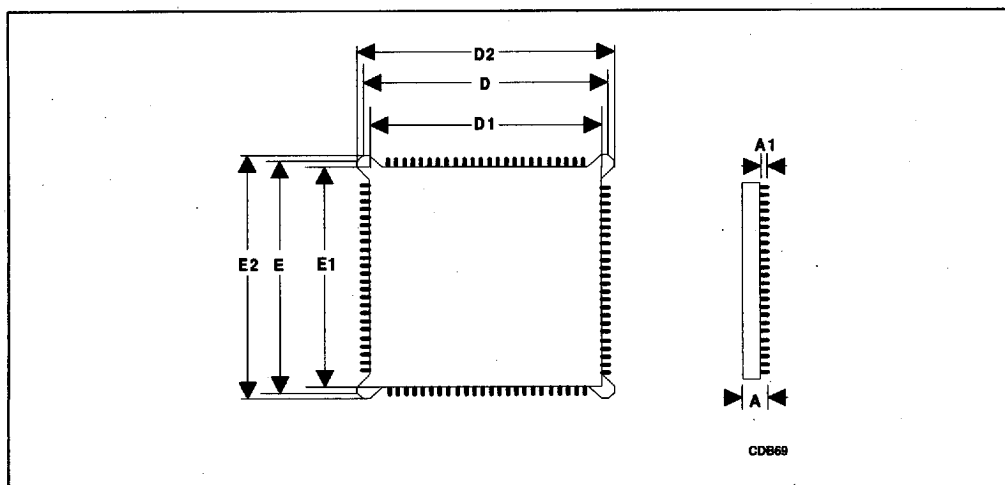
Figure 9-3. 82491 Cache SRAM Mechanical Specifications
