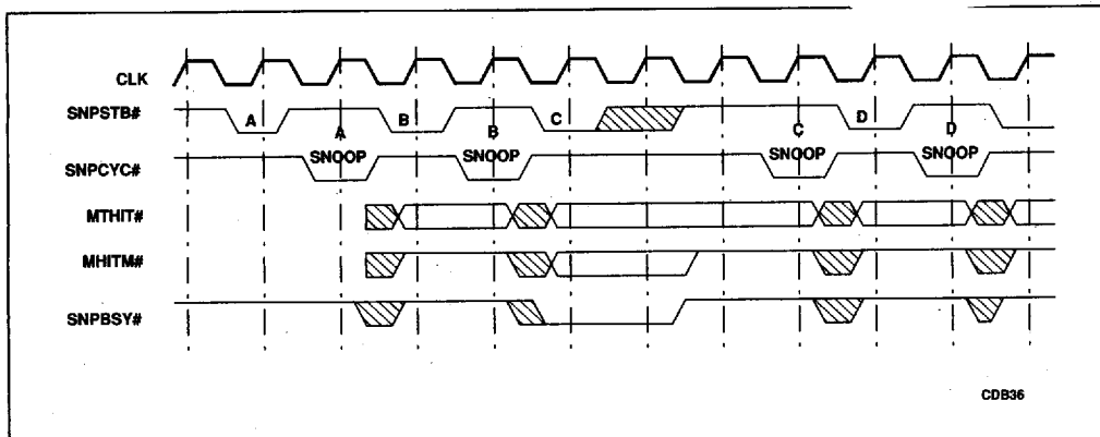
Figure 5-8. Fastest Synchronous Snooping
