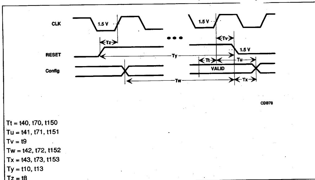
Figure 7-9. Reset and Configuration Timings
