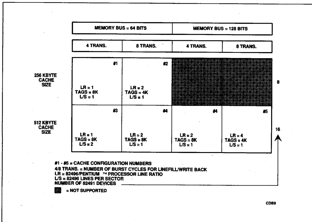
Figure 4-1. 82491 Cache Controller/82491 Cache SRAM Configurations with the Pentium™ Processor
