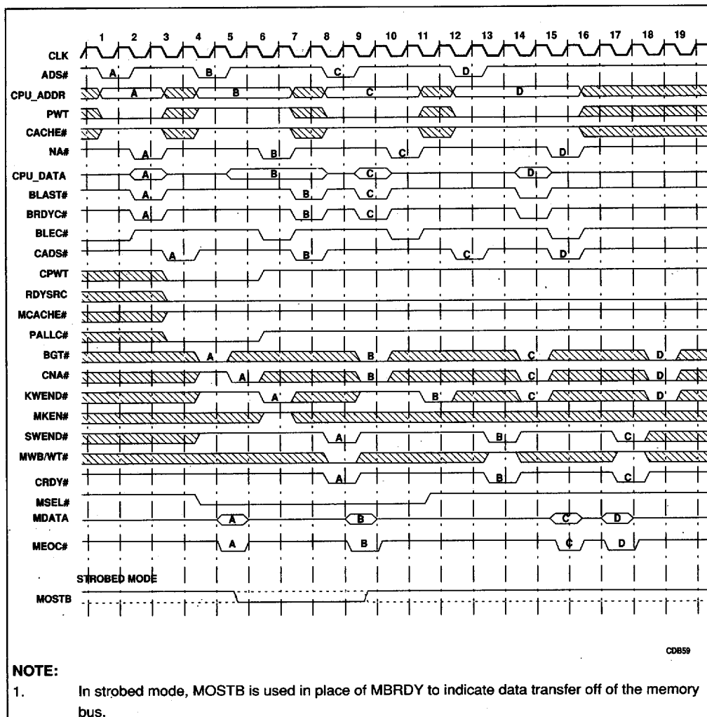
Figure 6-6. Write Miss with No Allocation or Write Hit to [S] State Cycles
