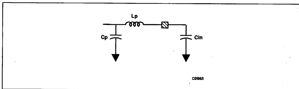
Figure 8-1. First Order Input Buffer
