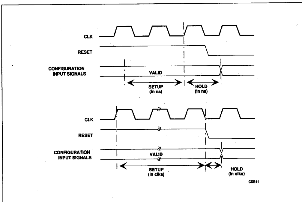
Figure 4-2. Configuration Input Sampling
