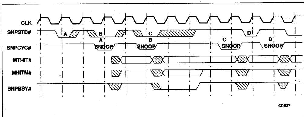
Figure 5-9. Fastest Asynchronous Snooping
