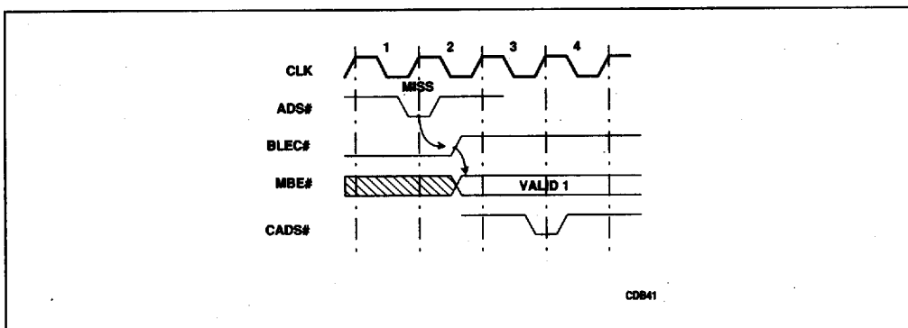
Figure 5-23. BLEC# Deassertion Due to ADS# Assertion
