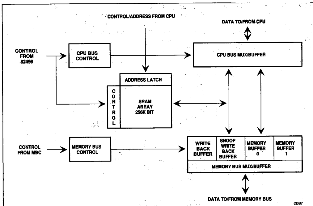
Figure 2-2. 82491 Cache SRAM Block Diagram
