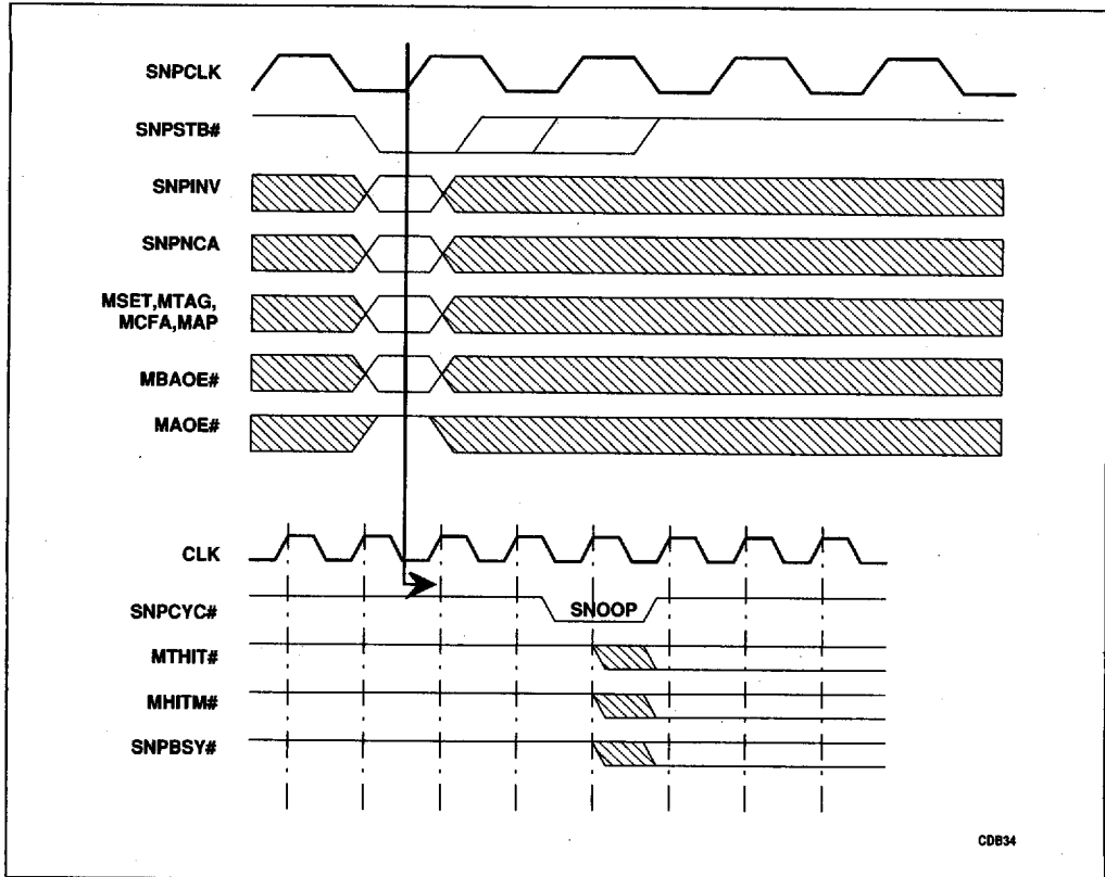
Figure 5-5. Clocked Snoop Mode
