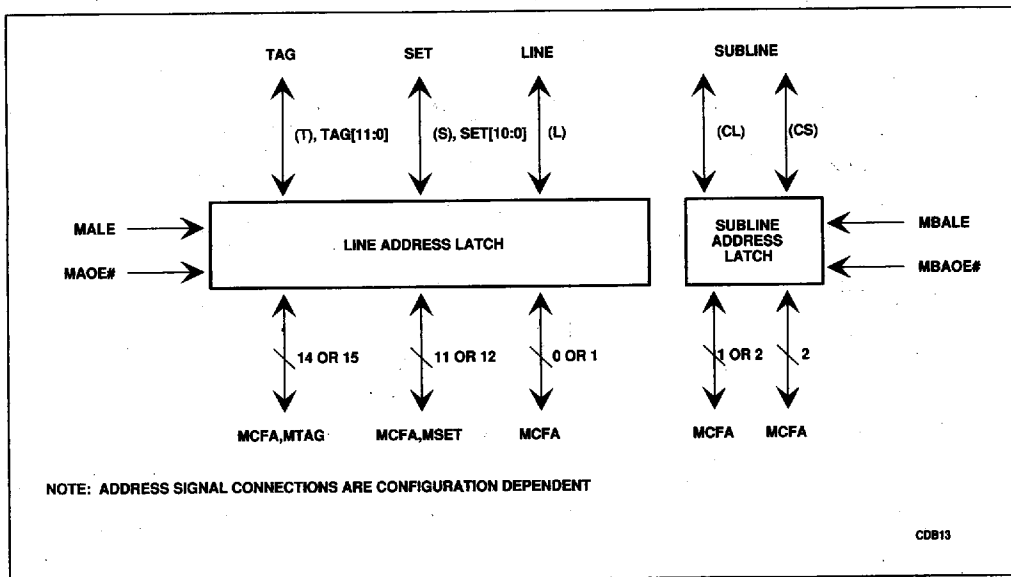
Figure 4-5. Address Latching
