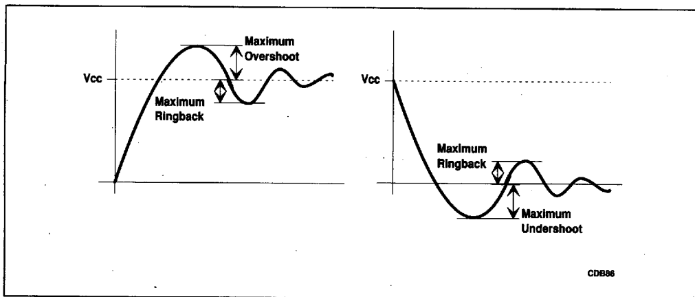
Figure 7-17. Overshoot/Undershoot and Ringback Guidelines
