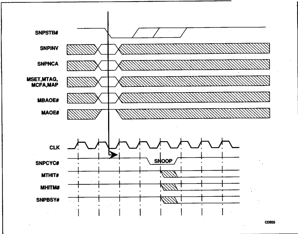
Figure 5-6. Strobed Snoop Mode
