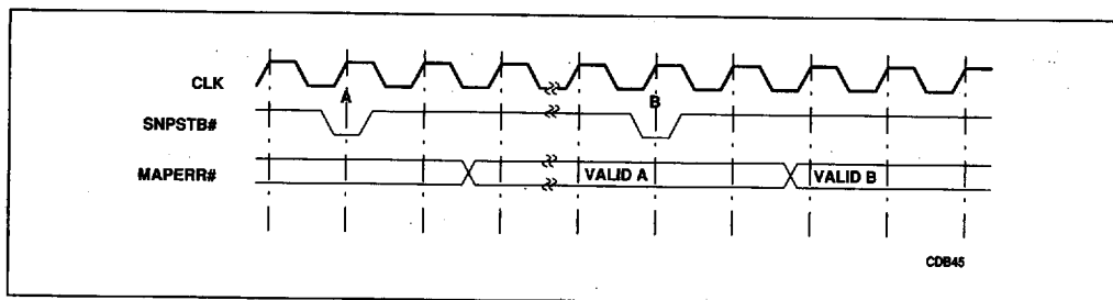
Figure 5-17. MAPERR# Timing for Synchronous Snoop Mode
