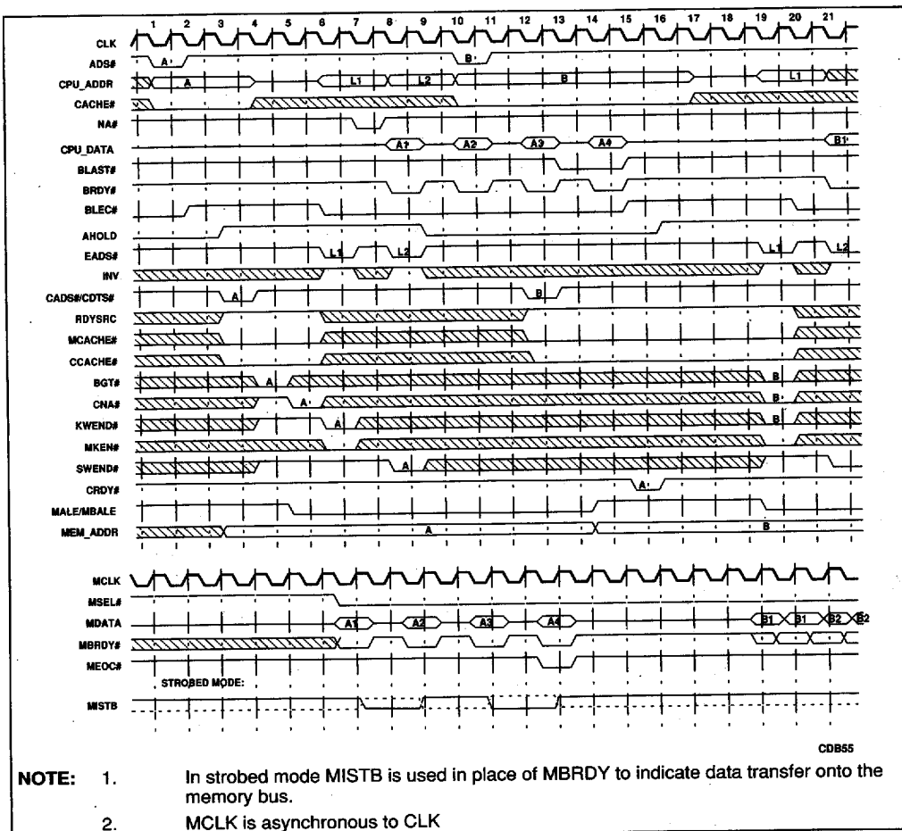
Figure 6-2. Read Miss With Clean Replacement
