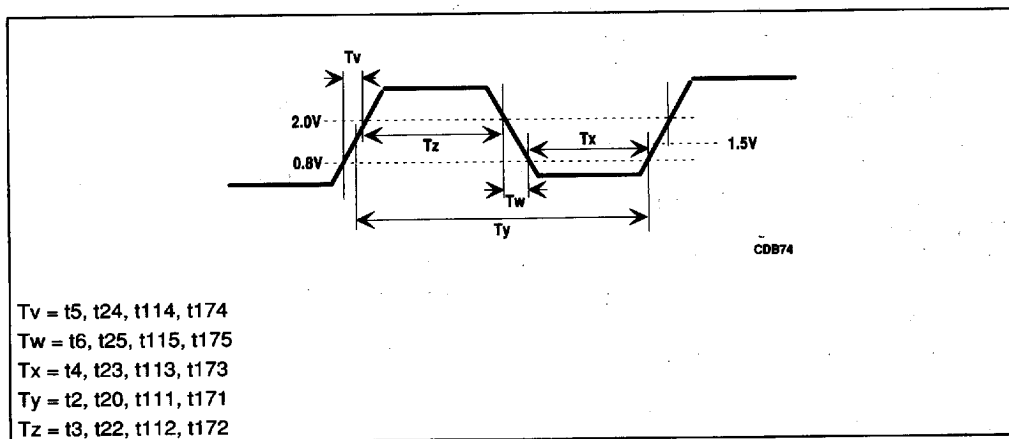
Figure 7-5. Clock Waveform
