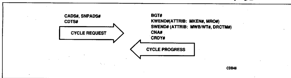
Figure 5-2. Memory Bus Cycle Progress and Attribute Signals
