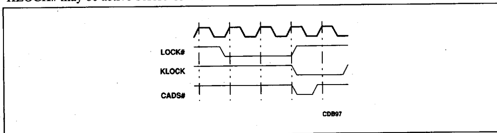
Figure 5-26. KLOCK# to LOCK# Relationship
