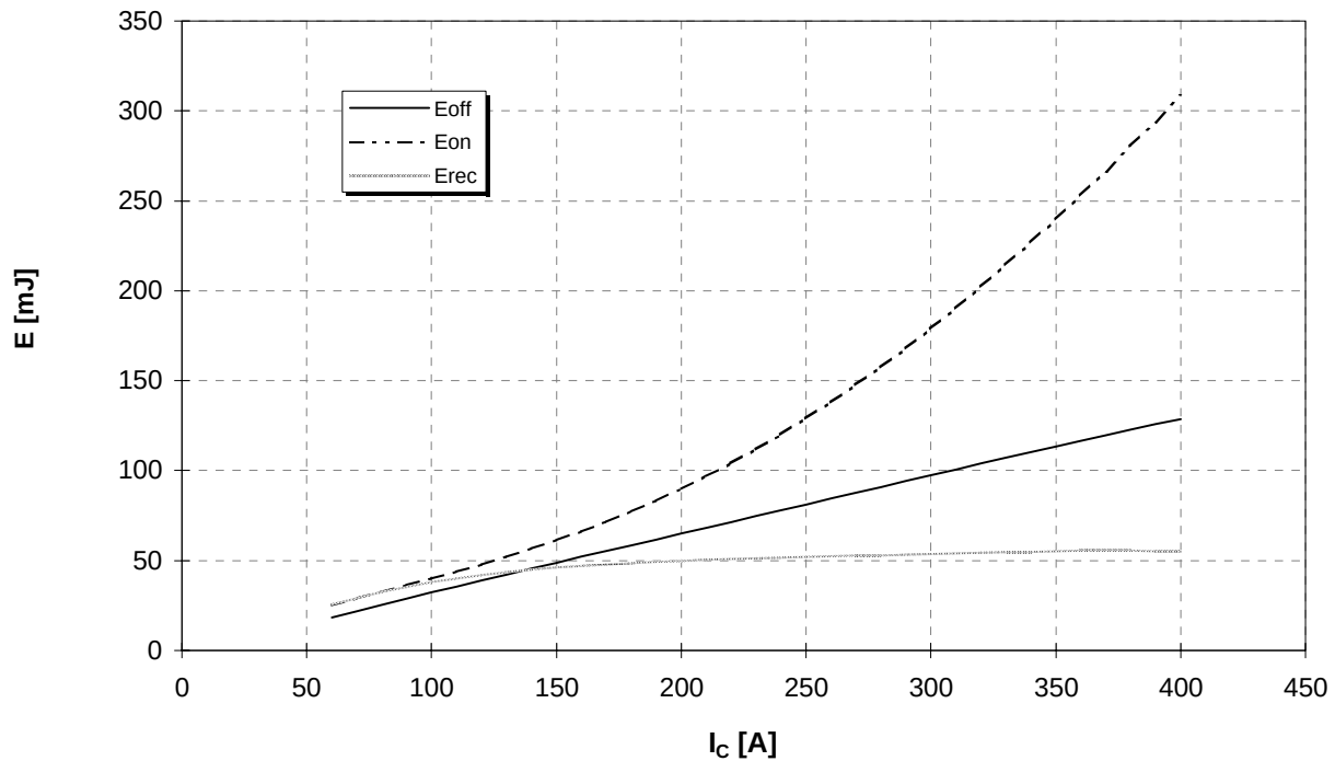
Schaltverluste (typisch) E_{on} = f(I_C) , E_{off} = f(I_C) , E_{rec} = f(I_C) Switching losses (typical) R_{gon} = R_{goff} = 7,5\Omega , V_{CE} = 900V , T_J = 125^\circ C
