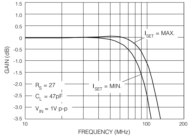
Fig. 3 I-SET Bandwidth vs Frequency
