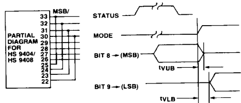
Figure 8. 8-Bit Bus Read Mode - 12-Bit Conversion
