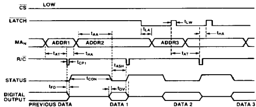
Figure 1. Timing for Bus Compatible DAS
