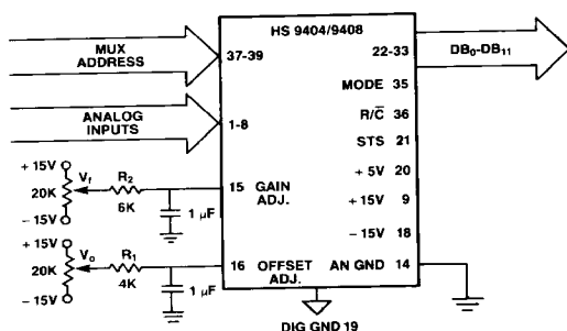
Figure 3. Gain and Offset Input Connections
