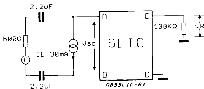
Figure 5 : Receiving Gain.
