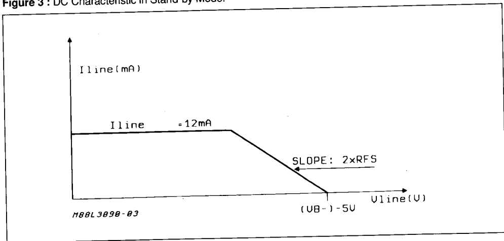
Figure 3 : DC Characteristic in Stand-by Mode.
