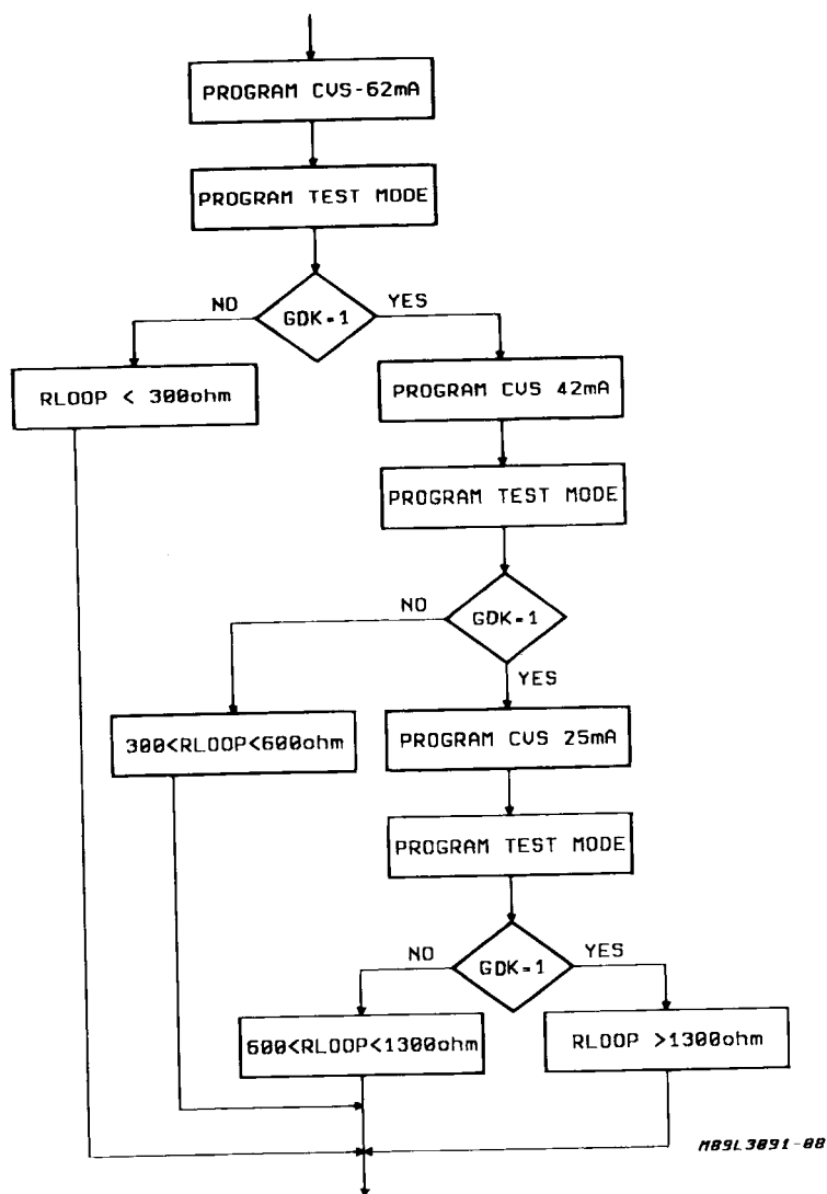
Figure 6 : Procedure for Loop Resistance Evaluation.
