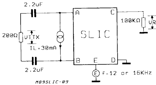
Figure 9 : TTX Level at Line Terminals.
