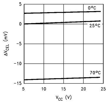
Output Voltage Regulation Vs V_{CC}
