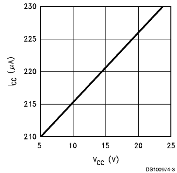
Quiescent Current Vs V_{CC}
