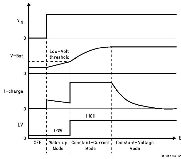
FIGURE 3. Typical Charge Cycle with Low-Voltage Detection Enabled.
