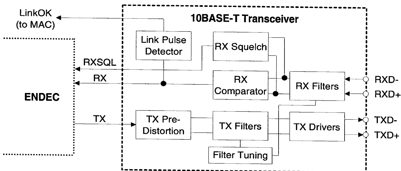
Figure 3.10. 10BASE-T Transceiver
