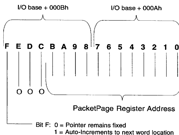
Figure 4.4. PackagePage Pointer
