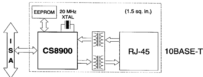
Figure 1.1. Complete Ethernet Motherboard Solution
