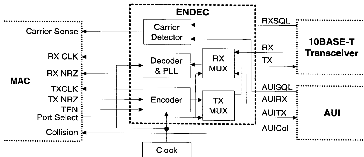
Figure 3.9. ENDEC
