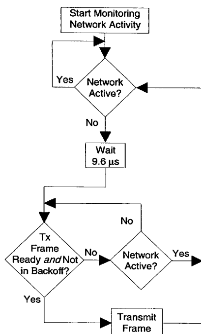
Figure 3.8. Simple Deferral
