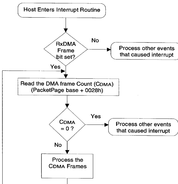
Figure 5.7. RxDMA Only Operation
