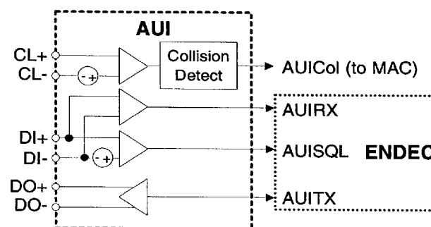
Figure 3.12. AUI
