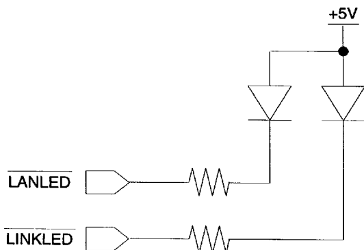
Figure 3.4. LED Connection Diagram
