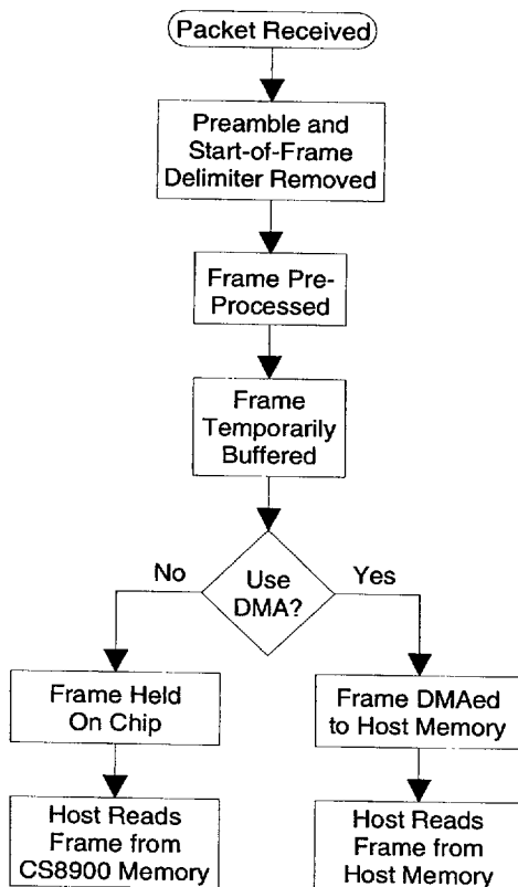
Figure 5.2. Frame Reception
