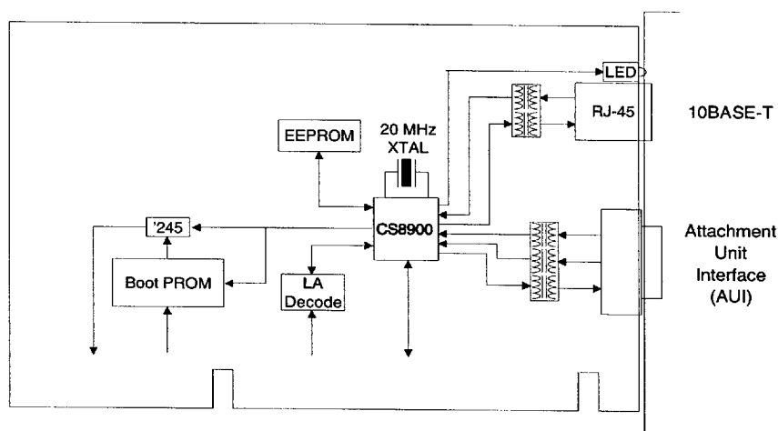
Figure 1.2. Full-Featured ISA Adapter Solution
