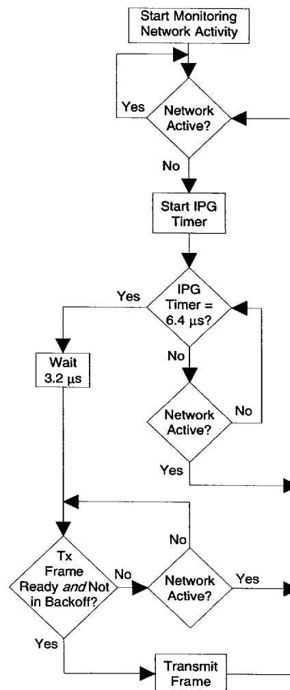
Figure 3.7. Two-Part Deferral
