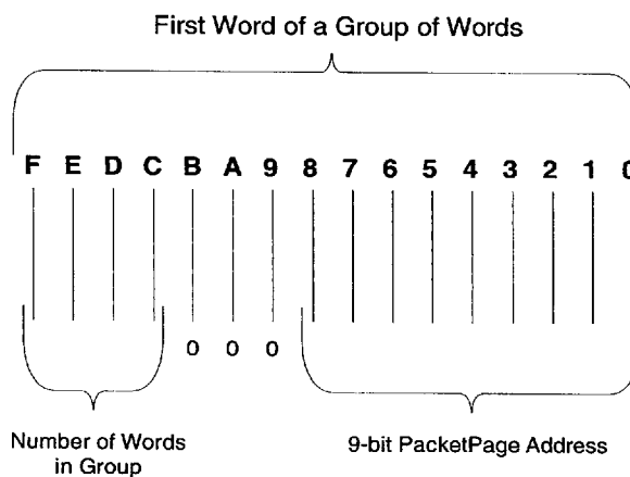
Figure 3.1. Group Header
