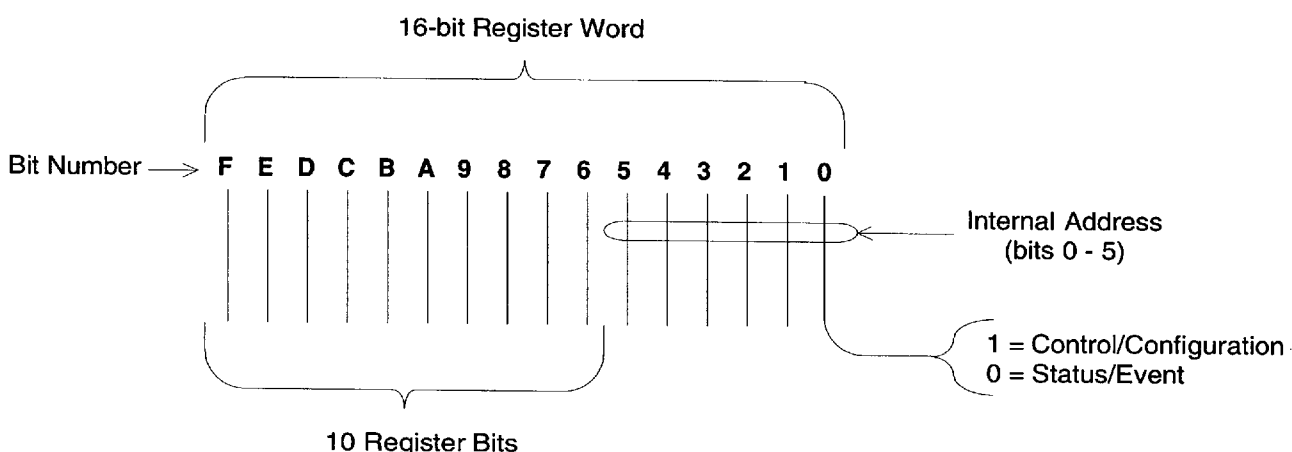
Figure 4.1. Status and Control Register Format
