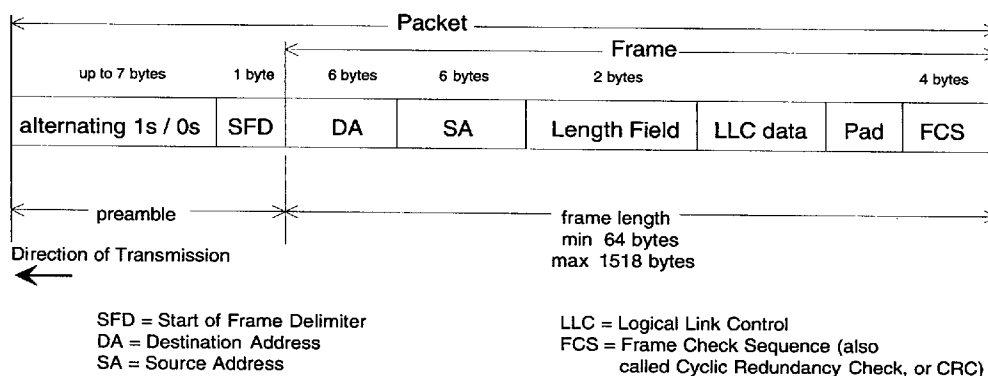
Figure 3.6. Ethernet Frame Format
