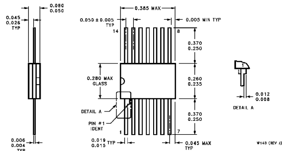
14-Lead Ceramic Flat Package (W) Order Number 5437FMBQ or DM5437W NS Package Number W14B
