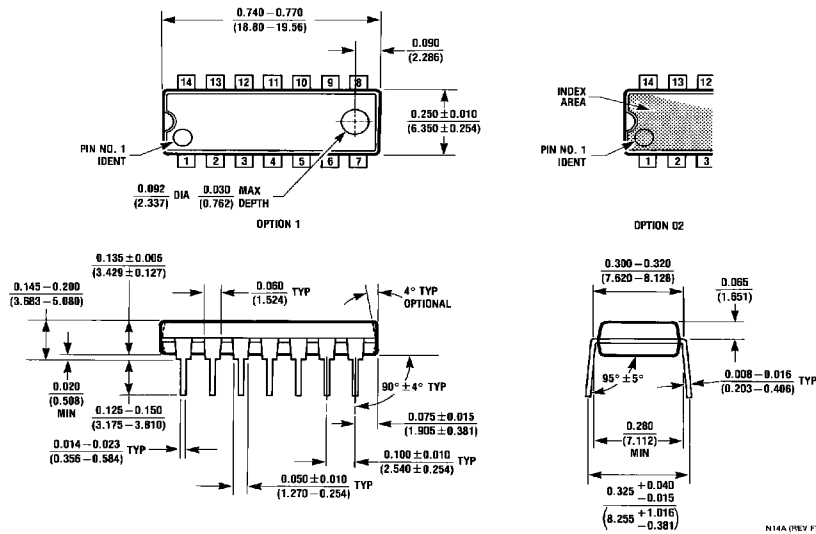
14-Lead Molded Dual-In-Line Package (N) Order Number DM7437N NS Package Number N14A
