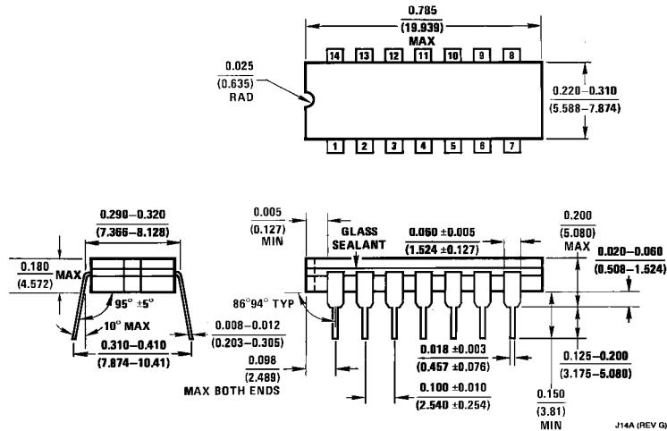
14-Lead Ceramic Dual-In-Line Package (J) Order Number 5437DMQB or DM5437J NS Package Number J14A
