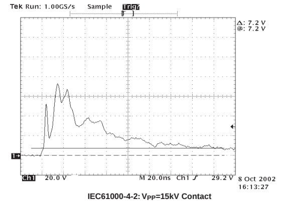
Fig. 8: ESD response @ V_{PP}=15\text{kV} contact.
