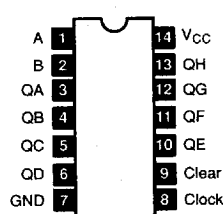
NTE74164, NTE74C164, NTE74HC164, NTE74LS164 14-Lead DIP, See Diag. 247 8-Bit Parallel-Out Serial Shift Register */Async Clear
