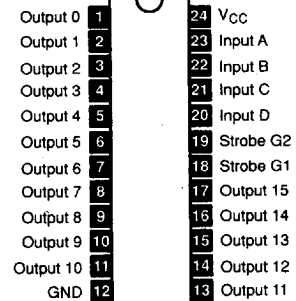
NTE74154, NTE74C154, NTE74HC154 24-Lead DIP, See Diag. 252 4-Line-to-16-Line Decoder/Demultiplexer
