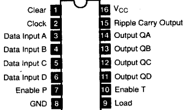
NTE74160, NTE74C160, NTE74LS160A, NTE74161, NTE74C161, NTE74HC161, NTE74HCT161, NTE74LS161A, NTE74162, NTE74LS162A, NTE74163, NTE74HC163, NTE74HCT163, NTE74LS163A, NTE74S163 16-Lead DIP, See Diag. 249 Synchronous 4-Bit Counter
