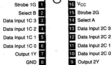
NTE74153, NTE74HC153, NTE74LS153, NTE74S153 16-Lead DIP, See Diag. 249 Dual 4-Line-to-1-Line Data Selector/Multiplexer
