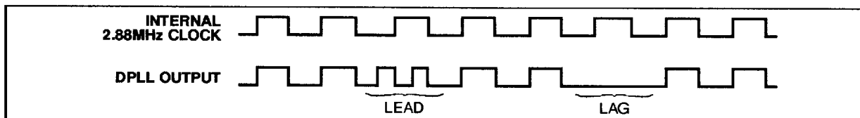
Figure 1 : DPLL Lead and Lag
