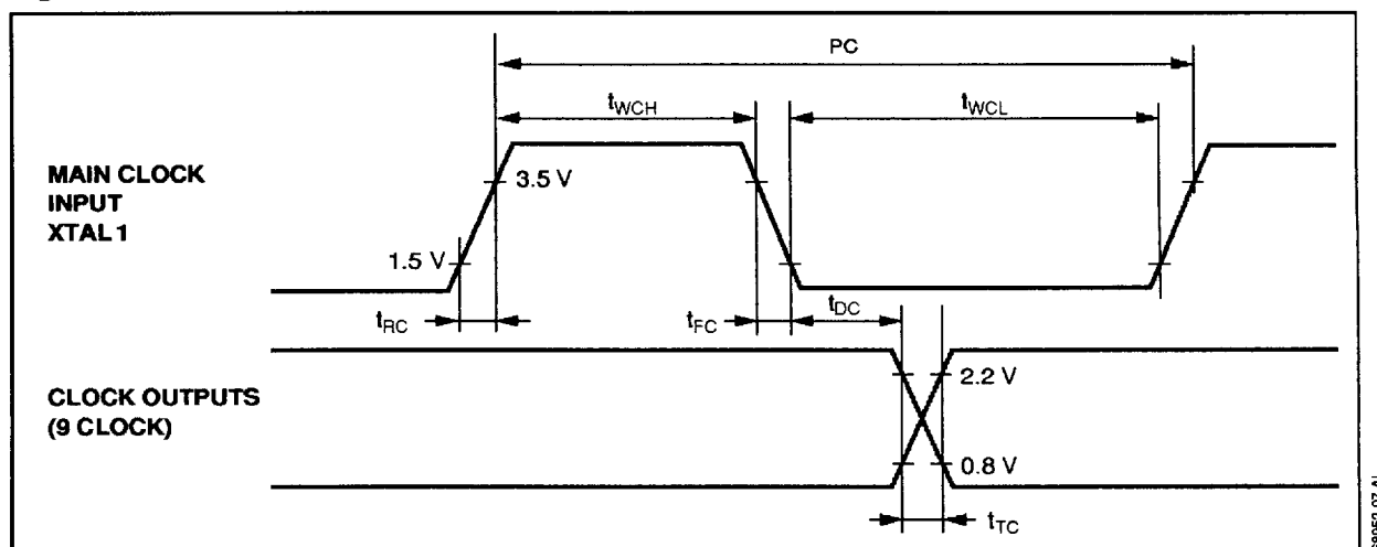
Figure 4 : Clock Wave Forms
