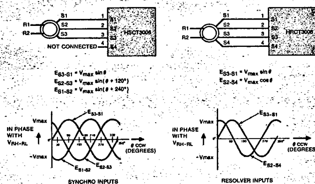
FIGURE 2 Synchro/Resolver Inputs
