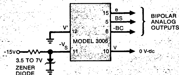
FIGURE 4 CONNECTIONS FOR BIPOLAR ANALOG OUTPUTS
