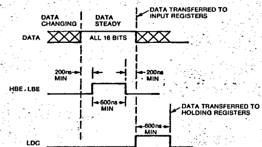
FIGURE 12 Single-Byte Loading
