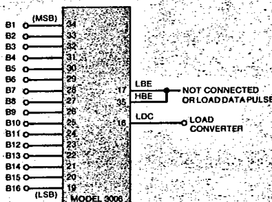
FIGURE 11 Digital Connections for One Byte (16 bits) Loading
