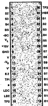
FIGURE 5 HSCT3006/HRCT3006 PIN ASSIGNMENTS
