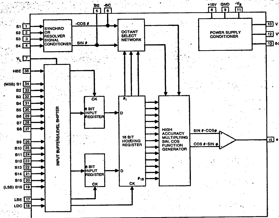
FIGURE 1 3006 BLOCK DIAGRAM
