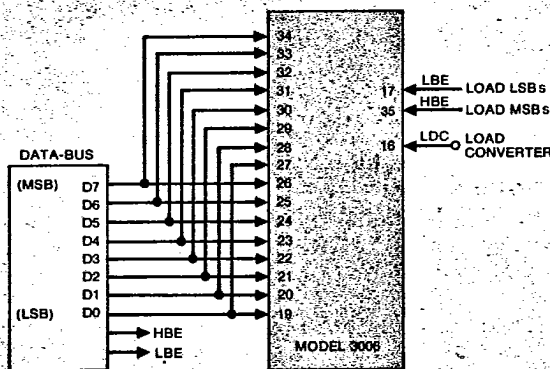
FIGURE 9 Digital Connections for Two-Byte Loading
