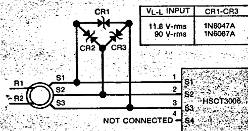
FIGURE 6 HSCT3006 Input Protection
