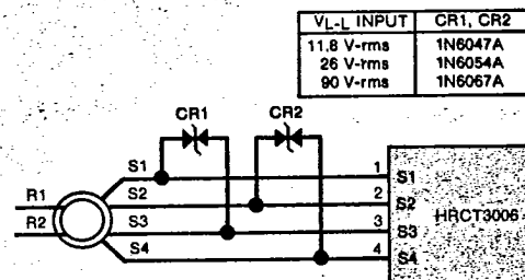
FIGURE 7 HRCT3006 Input Protection
