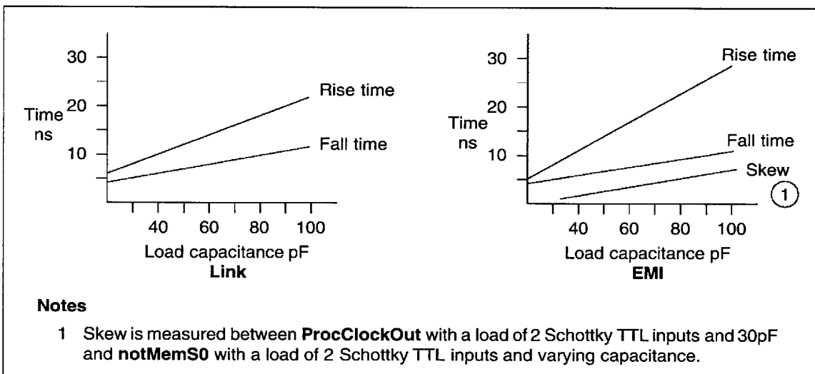
Figure 8.5 Typical rise/fall times
