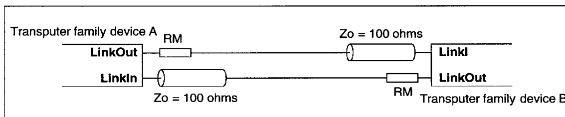
Figure 7.5 Links connected by transmission line
