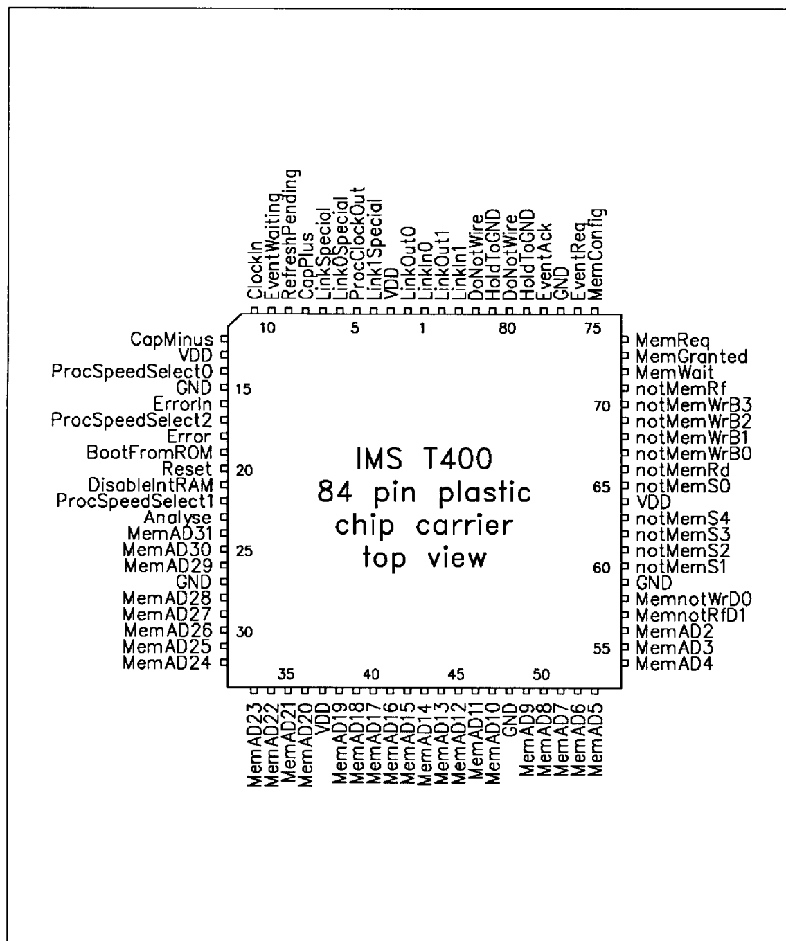
Figure 9.3 IMS T400 84-pin PLCC package pinout
