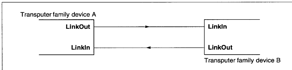
Figure 7.4 Links directly connected
