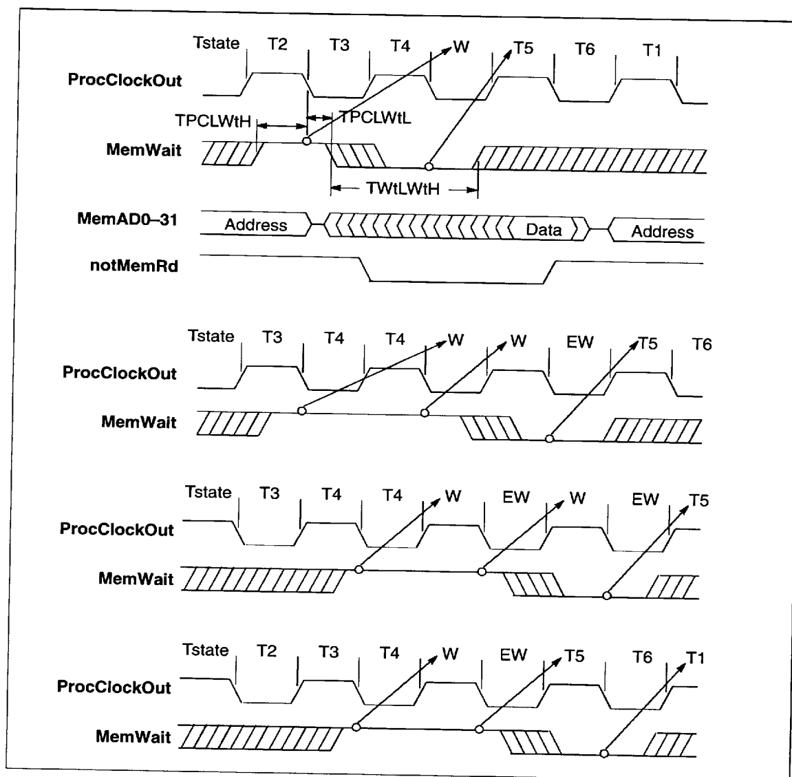
Figure 5.9 IMS T400 memory wait timing
