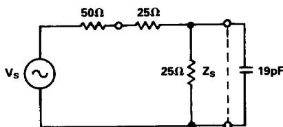
Figure 17a. Network for 50Ω Shunt Termination
