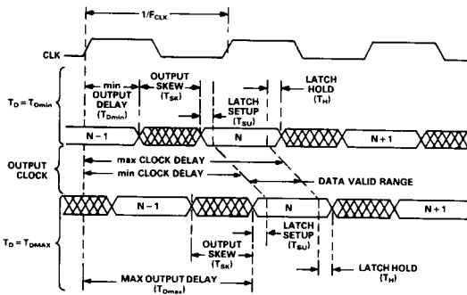
Figure 20. Detailed Timing Diagram Showing Output Delay Variation
