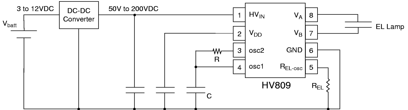
Figure 2: Pulsing EL Lamp
