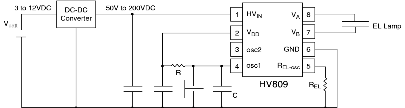
Figure 3: Push Button Delayed Turn Off
