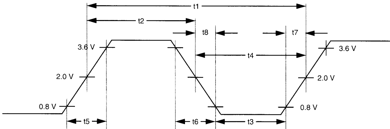
FIGURE 1. CLOCK WAVEFORMS
