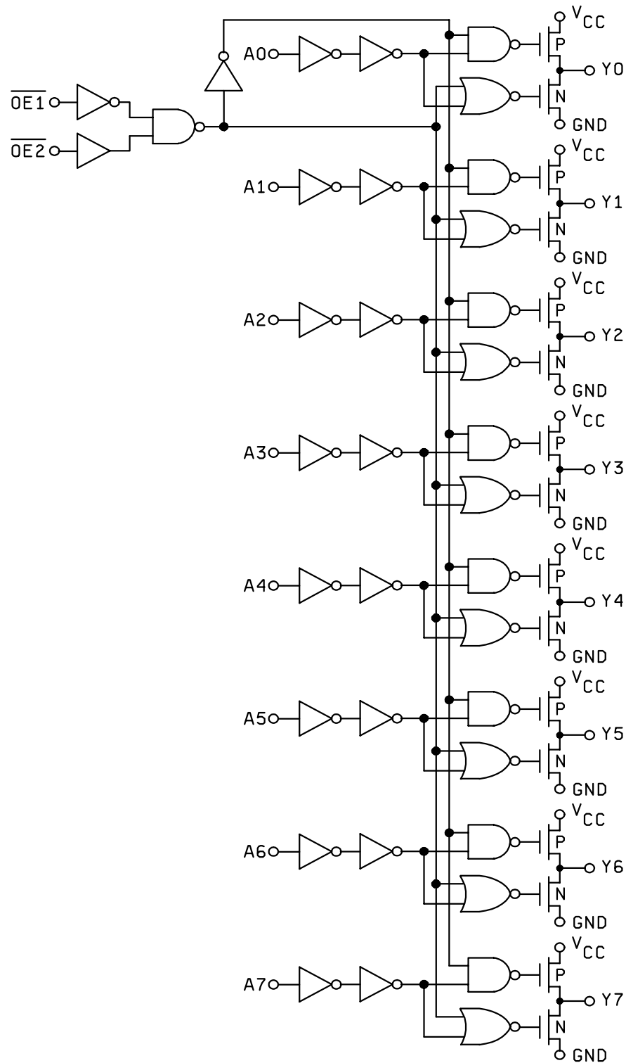
FIGURE 3. Logic diagram.
