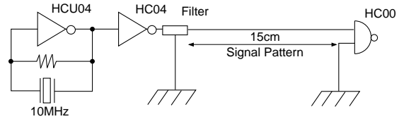
[Testing Circuit]
