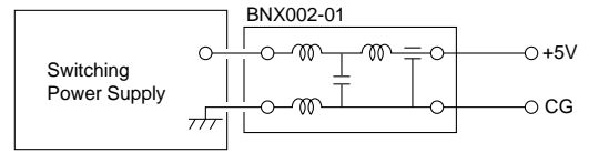
[Testing Circuit]
