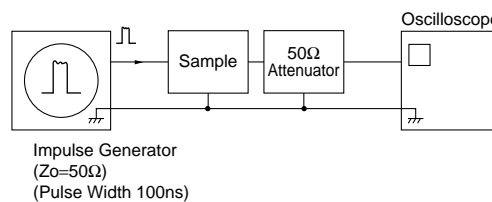
[TESTING CIRCUIT]
