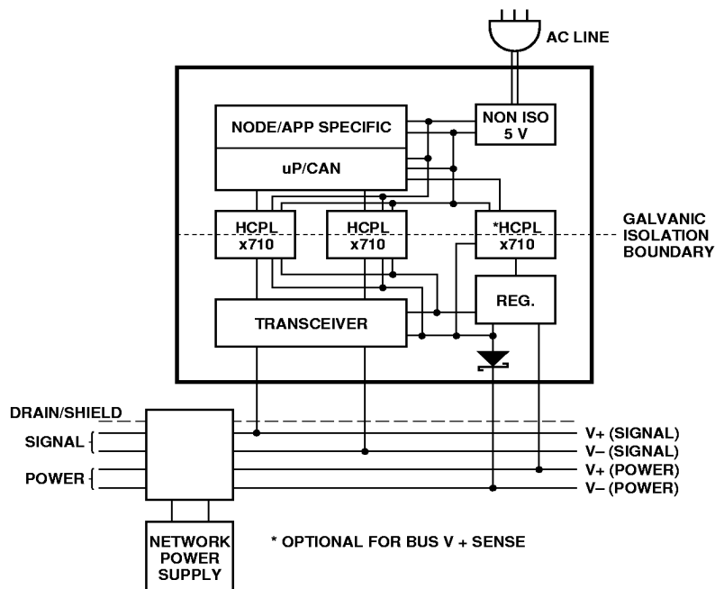
Figure 20. Isolated Node with Transceiver Powered by the Network.
