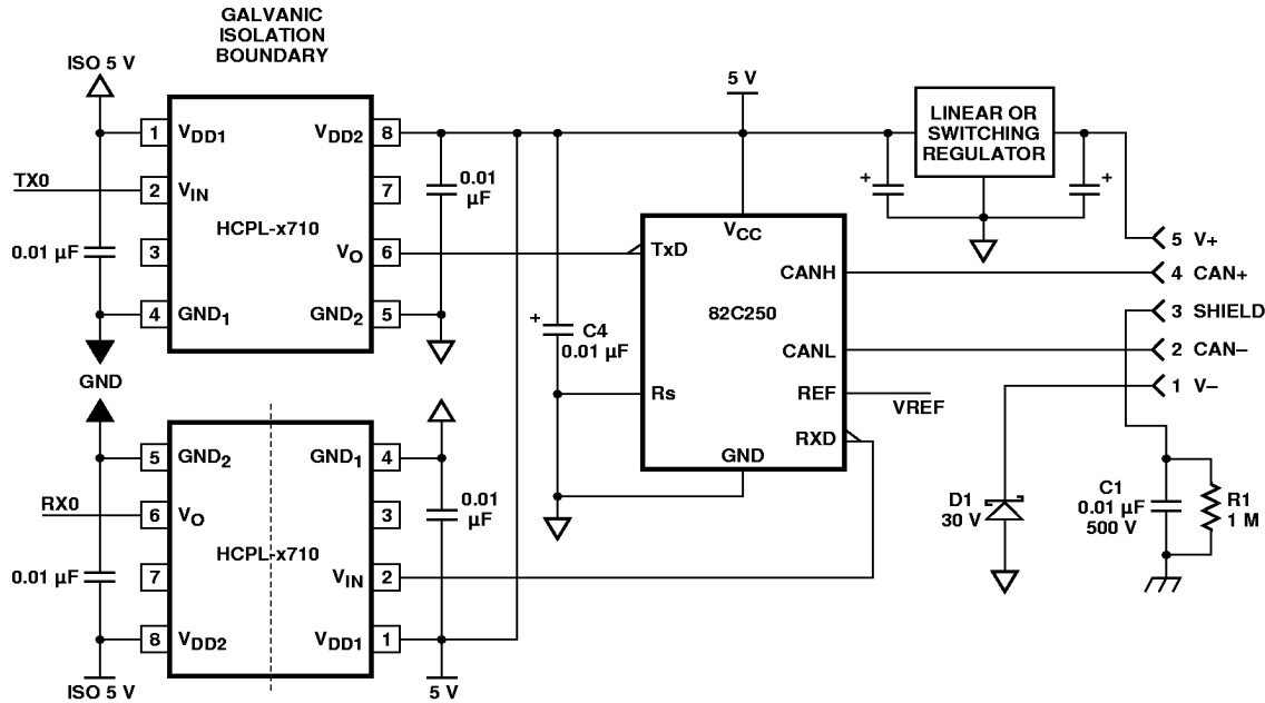
Figure 22. Recommended DeviceNet Application Circuit.
