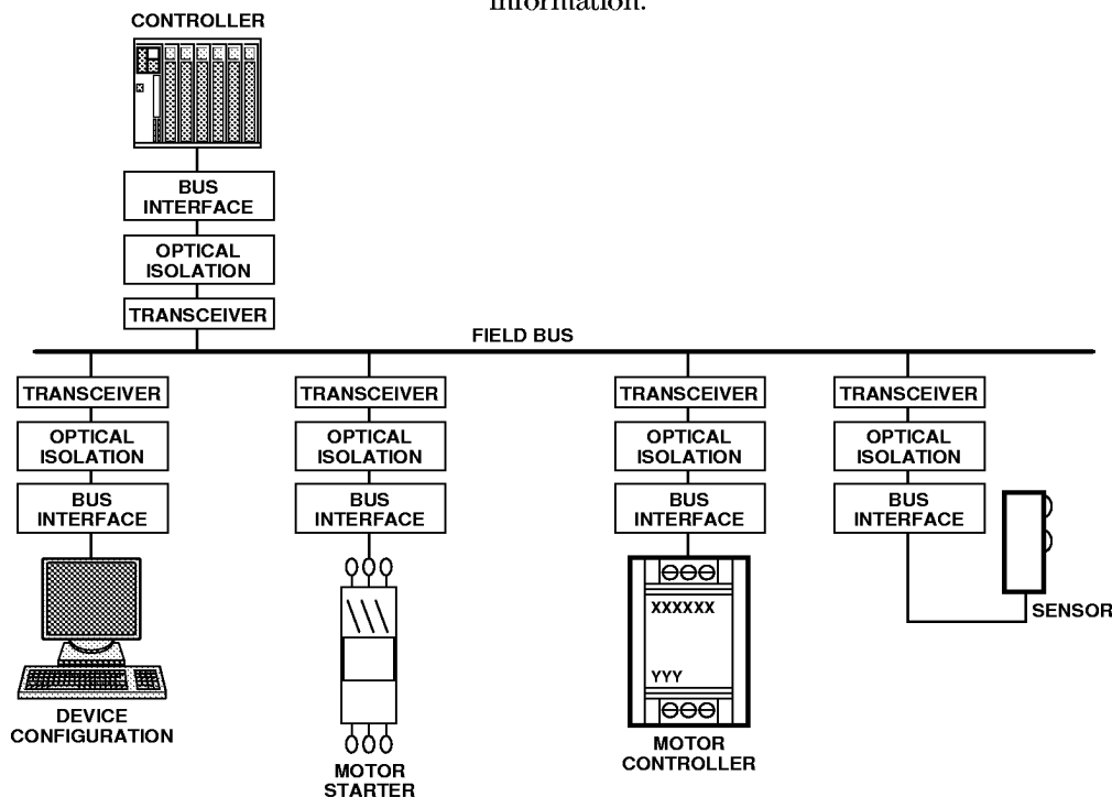
Figure 17. Typical Field Bus Communication Physical Model.
