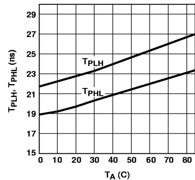
Figure 3. Typical Propagation Delays vs. Temperature.
