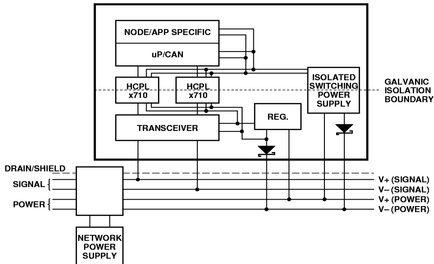
Figure 19. Isolated Node Powered by the Network.
