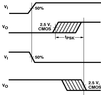
Figure 15. Propagation Delay Skew Waveform.
