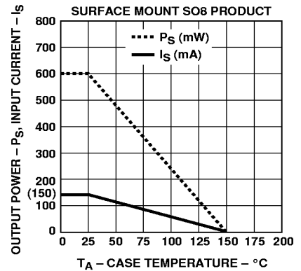
Figure 11. Thermal Derating Curve, Dependence of Safety Limiting Value with Case Temperature per VDE 0884.
