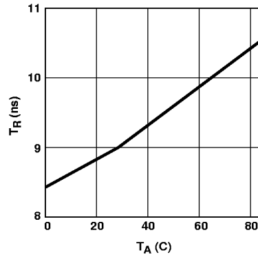
Figure 5. Typical Rise Time vs. Temperature.
