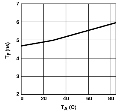
Figure 6. Typical Fall Time vs. Temperature.
