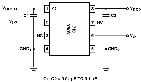
Figure 12. Recommended Printed Circuit Board Layout.
