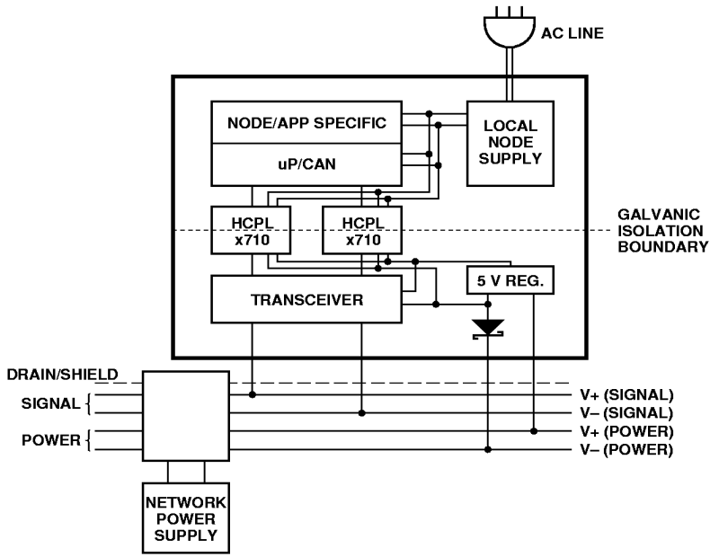
Figure 18. Typical DeviceNet Node.
