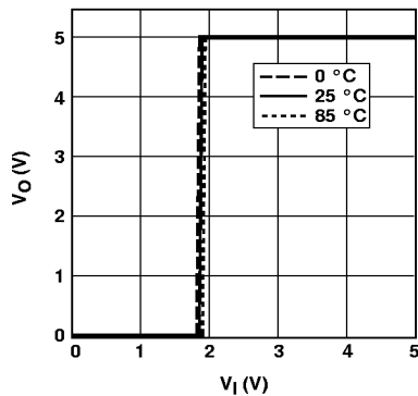
Figure 1. Typical Output Voltage vs. Input Voltage.
