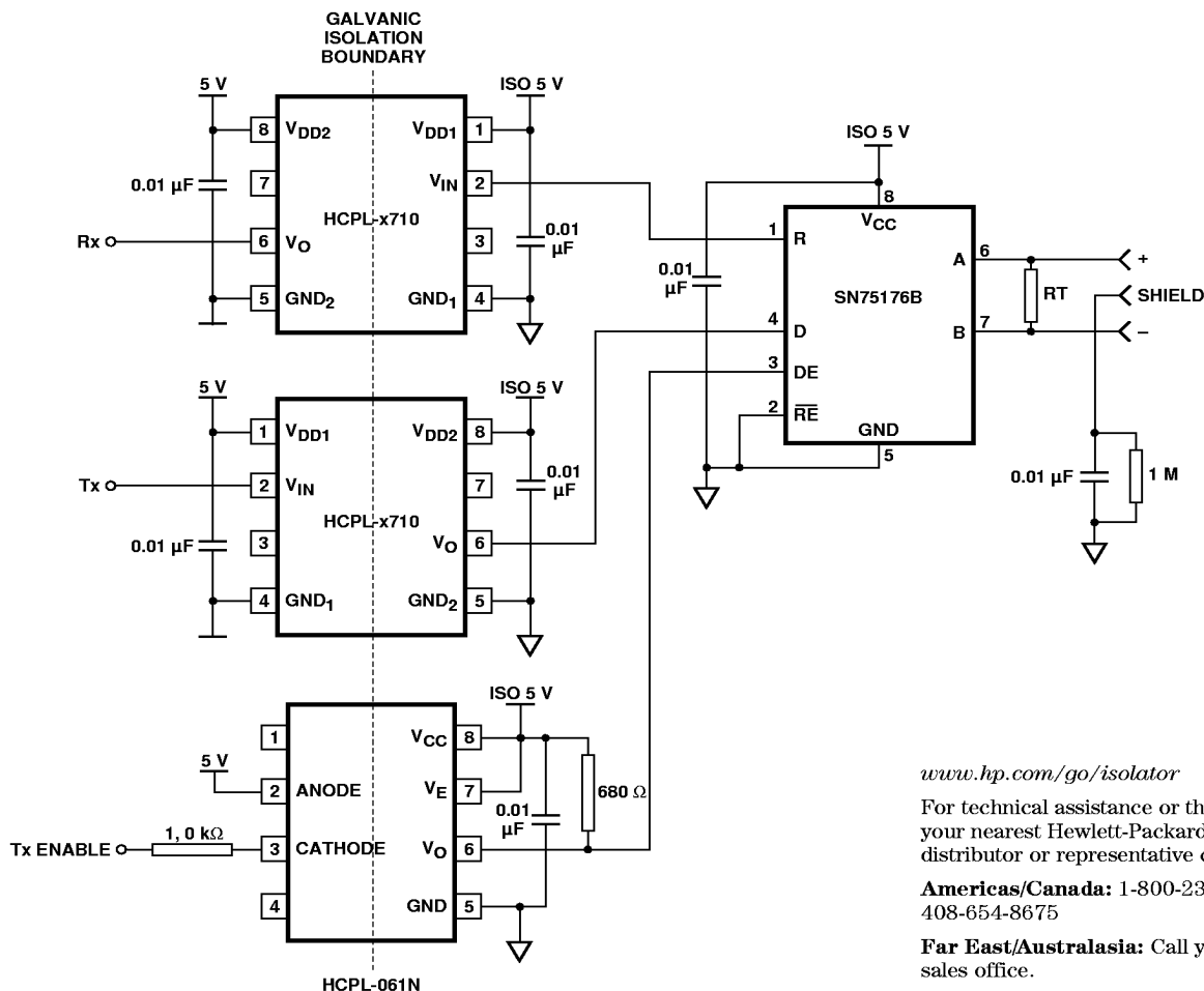
Figure 24. Recommended PROFIBUS Application Circuit.
