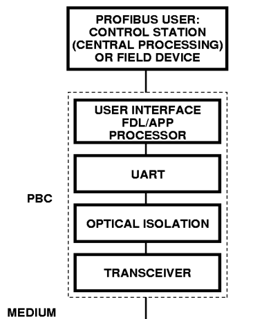
Figure 23. PROFIBUS Controller (PBC).
