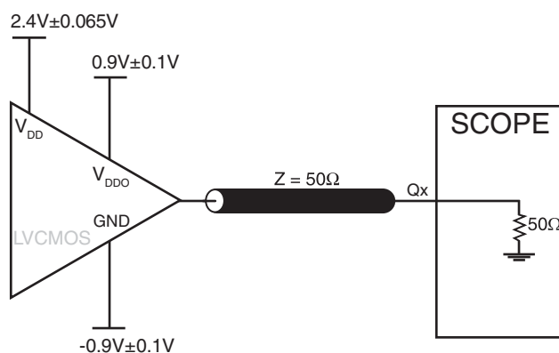
3.3V CORE/1.8V OUTPUT LOAD AC TEST CIRCUIT
