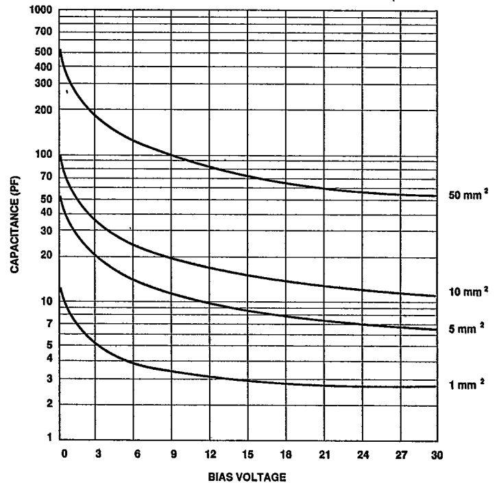
Fig.14 SERIES 0 - TYPICAL CAPACITANCE VERSUS BIAS VOLTAGE FOR A GIVEN DETECTOR AREA
