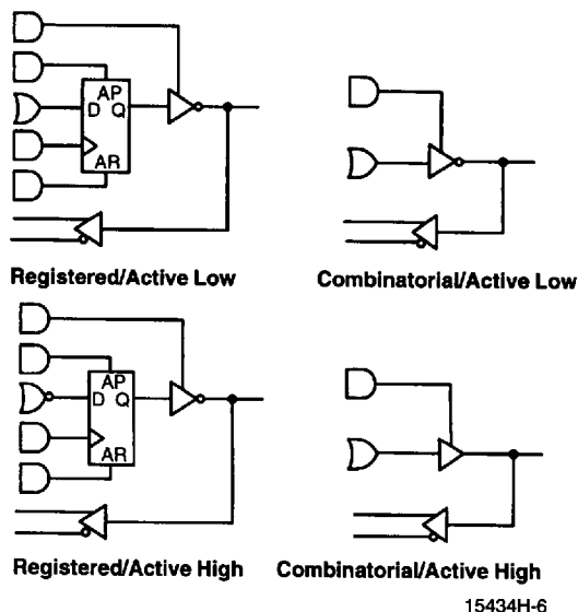
Figure 2. Macrocell Configurations
