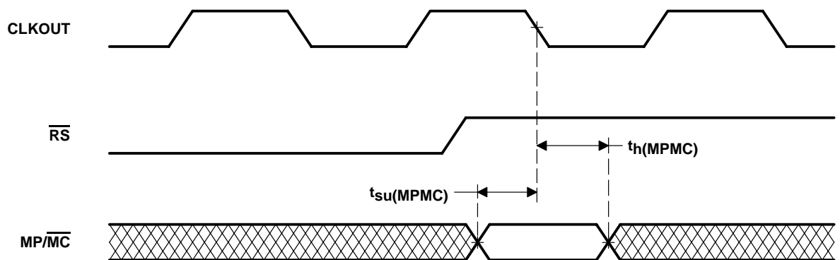
Figure 5–17. \overline{\text{MP/MC}} Timing
