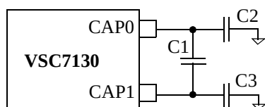
Figure 4: Loop Filter Capacitors (Recommended Circuit)
