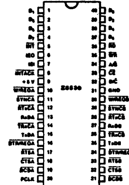
DEP Pin Assignments: Z8530
