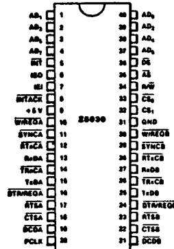
DIP Pin Assignments, 28030
