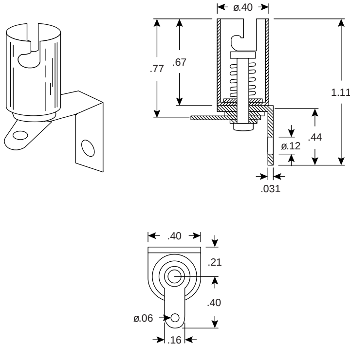
Dimensions (In.)
