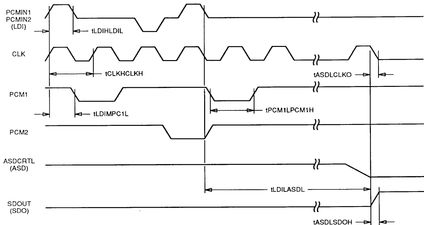
Figure 4. Normal Mode I/O Format
