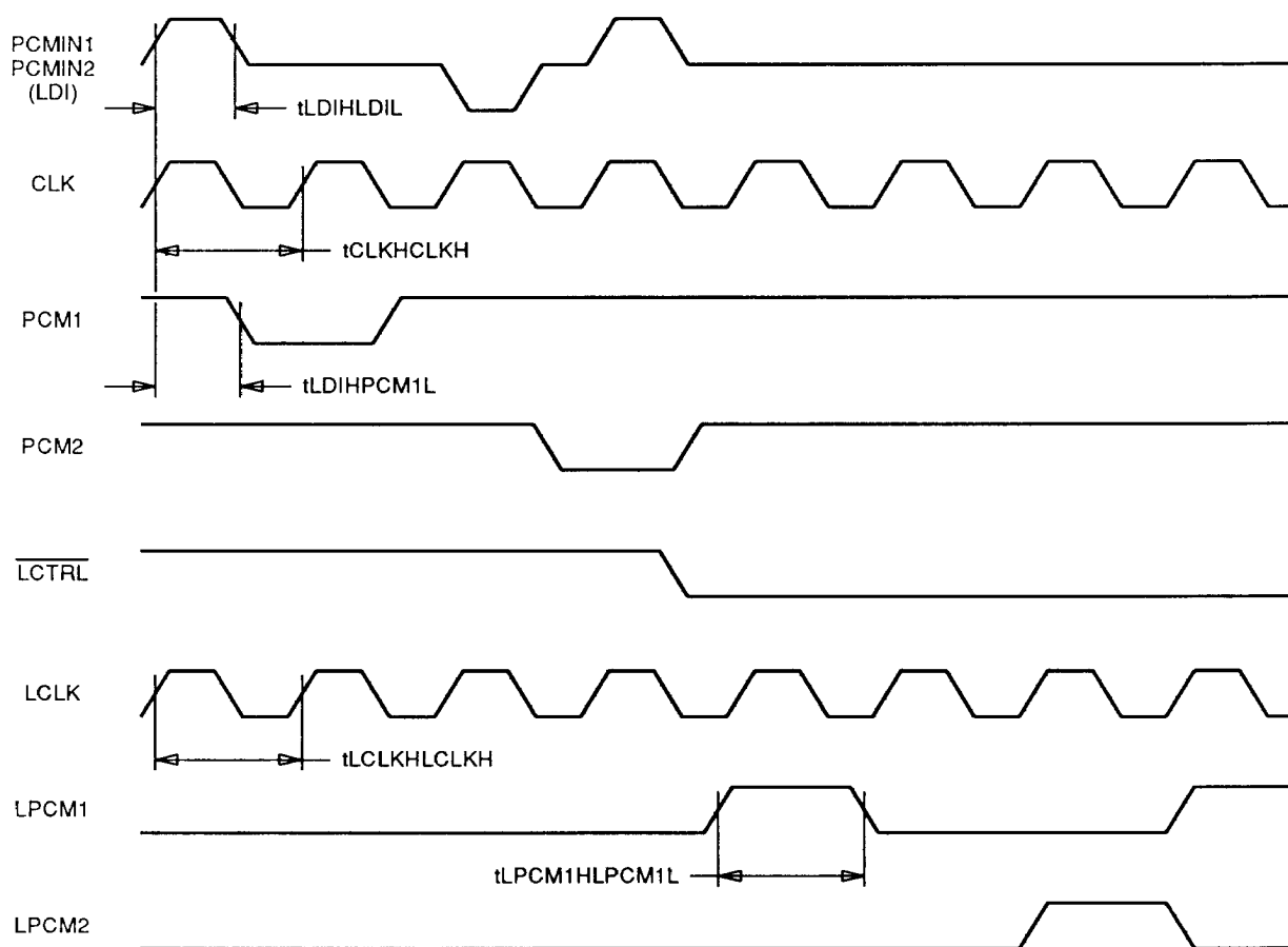
Figure 5. Loopback Mode I/O Format
