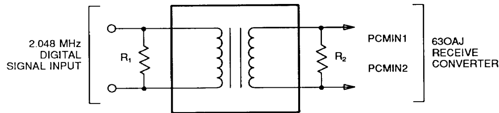
Figure 3. Transformer and Resistor Network
