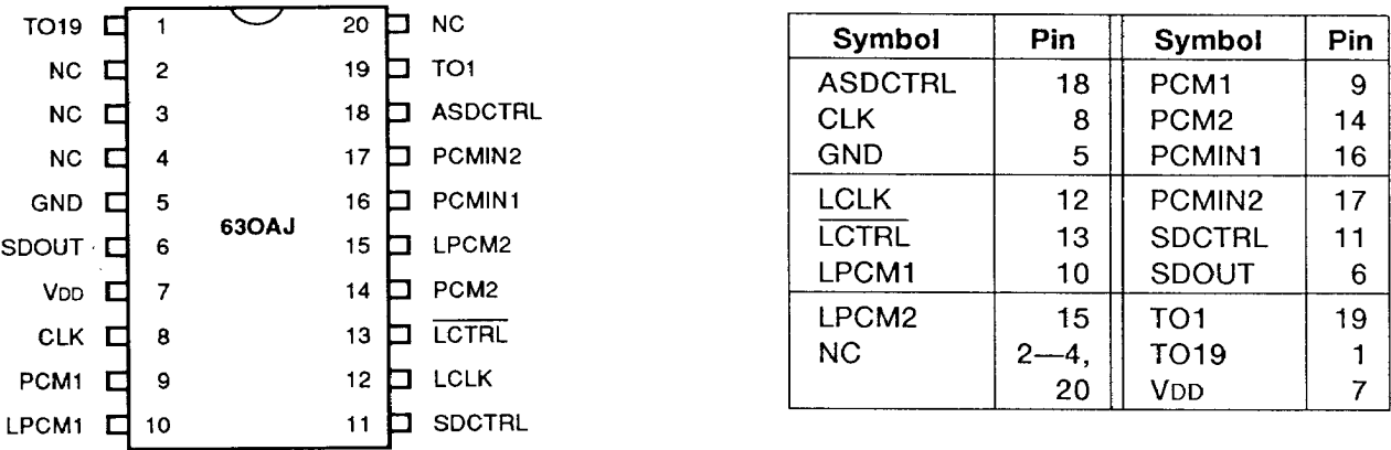
Figure 2. Pin Function Diagram and Alphabetical Listing of Symbols
