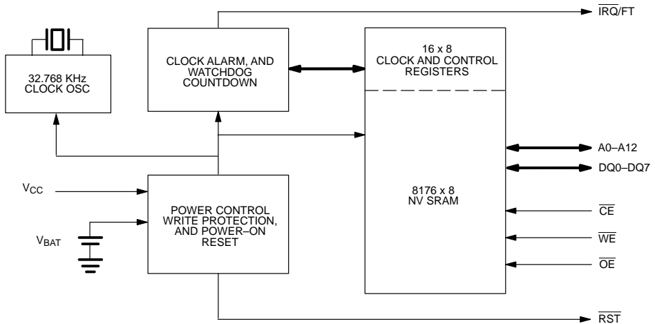
DS1543 BLOCK DIAGRAM Figure 1
