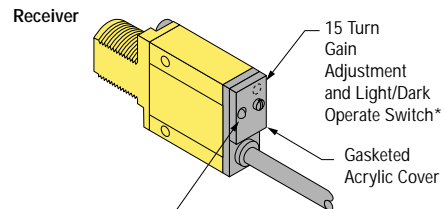
"AID" Indicator LED lights when the sensor sees the reflection of its own modulated light and pulses at a rate proportional to the strength of the received light signal
