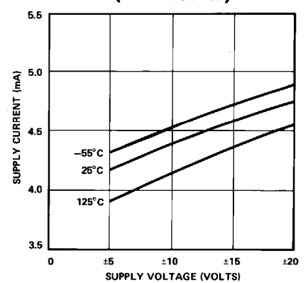
SUPPLY CURRENT vs SUPPLY VOLTAGE (OP-16/OP-17)
