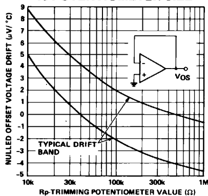
NULLED OFFSET VOLTAGE DRIFT vs POTENTIOMETER SIZE
