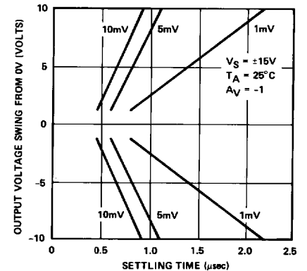
SETTLING TIME
