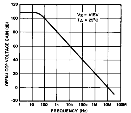
OPEN-LOOP GAIN vs FREQUENCY
