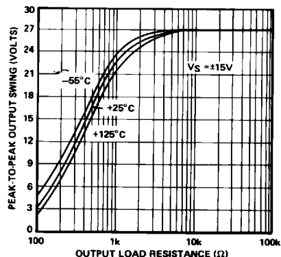
MAXIMUM OUTPUT SWING vs LOAD RESISTANCE
