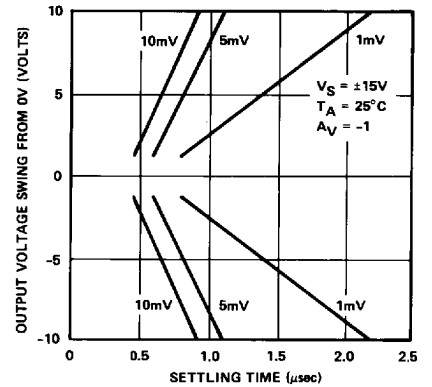
SETTLING TIME
