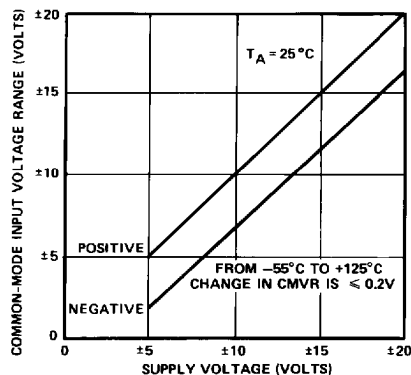
COMMON-MODE INPUT VOLTAGE RANGE vs SUPPLY VOLTAGE
