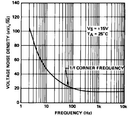
VOLTAGE NOISE vs FREQUENCY
