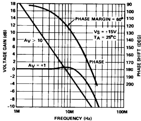
CLOSED-LOOP BANDWIDTH AND PHASE SHIFT vs FREQUENCY
