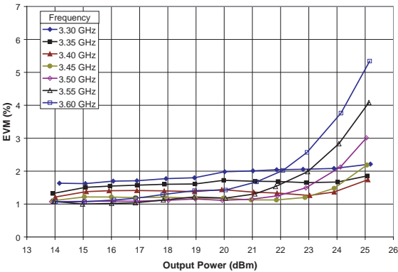
Figure 5: Uncorrected EVM vs. Output Power (T C = +25 °C, V CC = +6.0 V, V BIAS = +3.0 V, 54 Mbps OFDM Modulation, system EVM Approx. 0.8 %)
