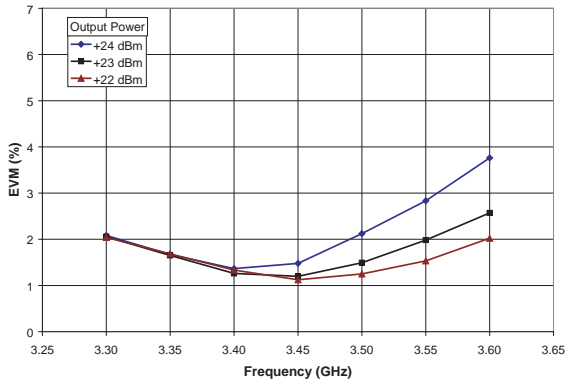
Figure 6: Uncorrected EVM vs. Frequency (T C = +25 °C, V CC = +6.0 V, V BIAS = +3.0 V, 54 Mbps OFDM Modulation, system EVM Approx. 0.8 %)
