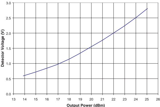
Figure 7: Detector Voltage vs. Output Power (T C = +25 °C, V CC = +6.0 V, V BIAS = +3.0 V, f = 3.5 GHz, 54 Mbps OFDM Modulation)
