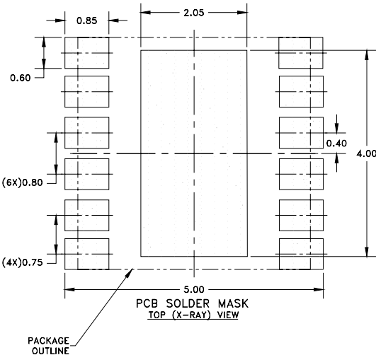
Figure 17: Land Pattern
