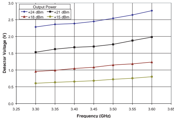
Figure 8: Detector Voltage vs. Frequency (T C = +25 °C, V CC = +6.0 V, V BIAS = +3.0 V, 54 Mbps OFDM Modulation)
