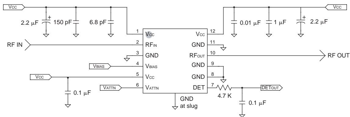
Figure 16: Application Circuit
