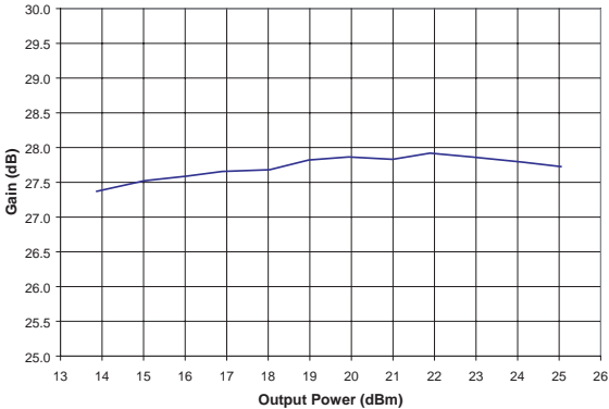
Figure 3: Gain vs. Output Power (T C = +25 °C, V CC = +6.0 V, V BIAS = +3.0 V, f = 3.5 GHz, 54 Mbps OFDM Modulation)
