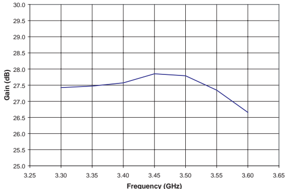
Figure 4: Gain vs. Frequency (T C = +25 °C, V CC = +6.0 V, V BIAS = +3.0 V, P OUT = +24 dBm, 54 Mbps OFDM Modulation)
