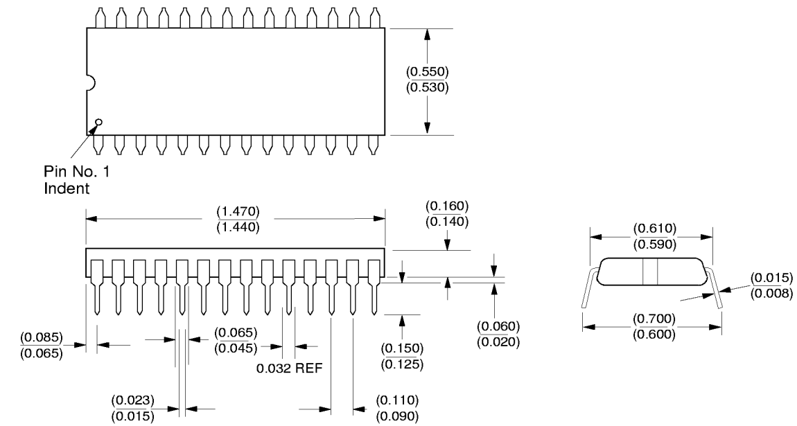
28-Pin Plastic Dip
