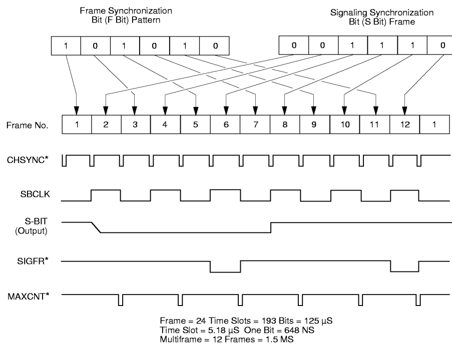
F Bit ( F_T ) Alignment Signal (Odd-Numbered Frames)
