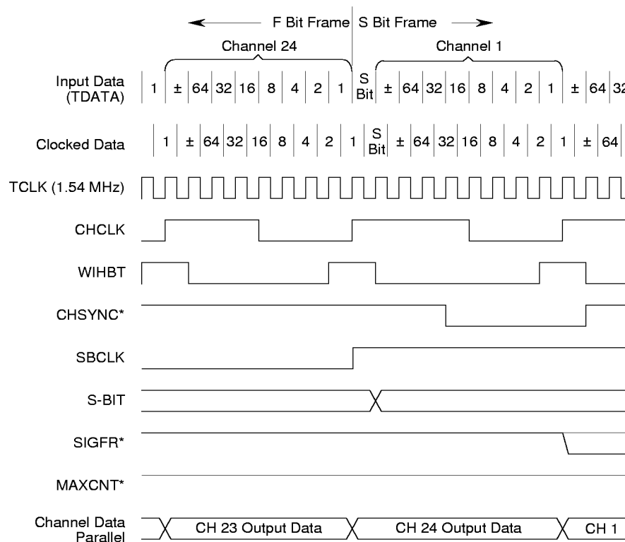
Figure 2. Signal Relationships at Beginning of F_S Frame (S-BIT).
