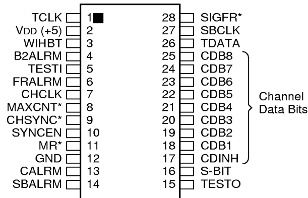
Figure 1. Pin Configuration.
