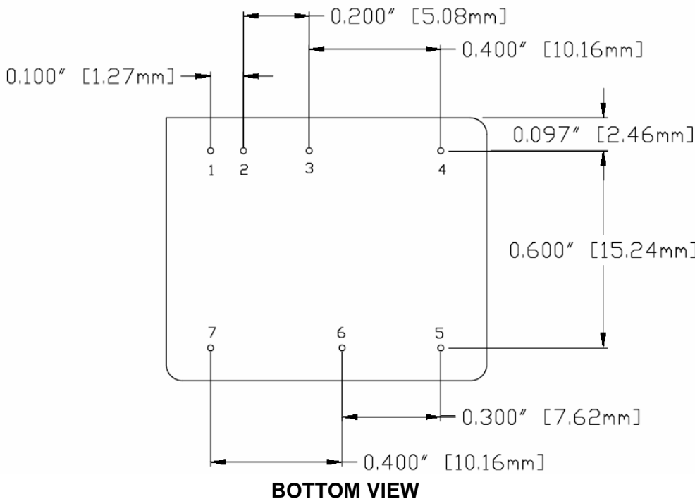
Figure 12 – Package and Pinout (Dimensional Limits are ±0.005" Unless Otherwise Stated)
