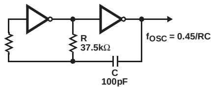
FIGURE 12. CMOS OSCILLATOR
