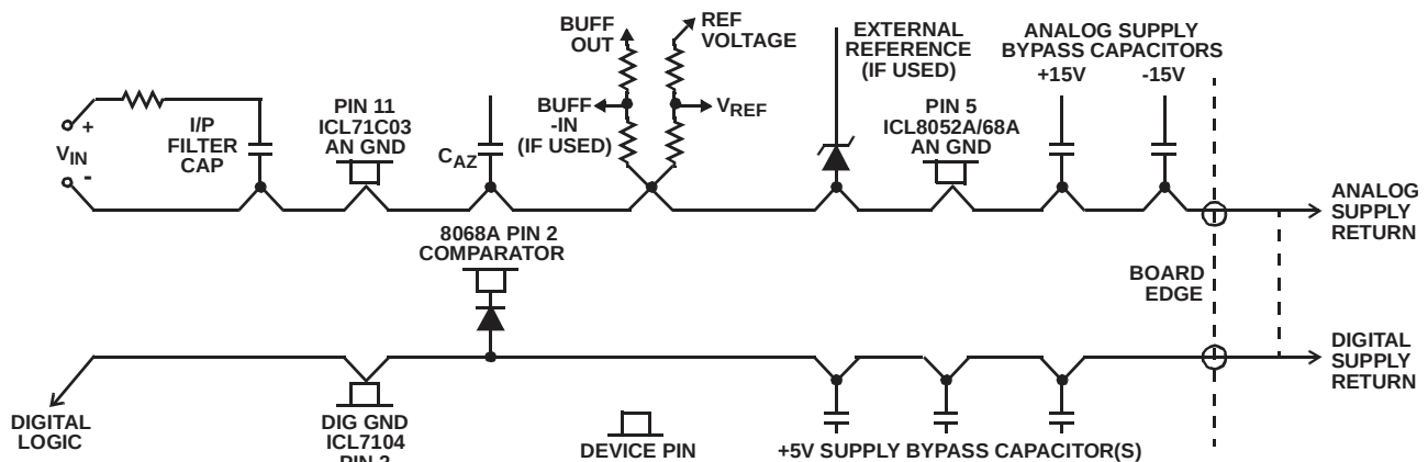
FIGURE 9. GROUNDING SEQUENCE
