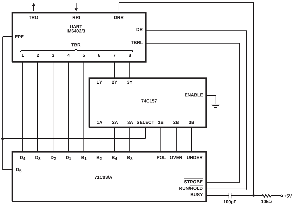
FIGURE 16. COMPLEX ICL71C03/71C03A TO UART INTERFACE
