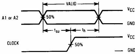
Figure 3. Switching Waveforms
